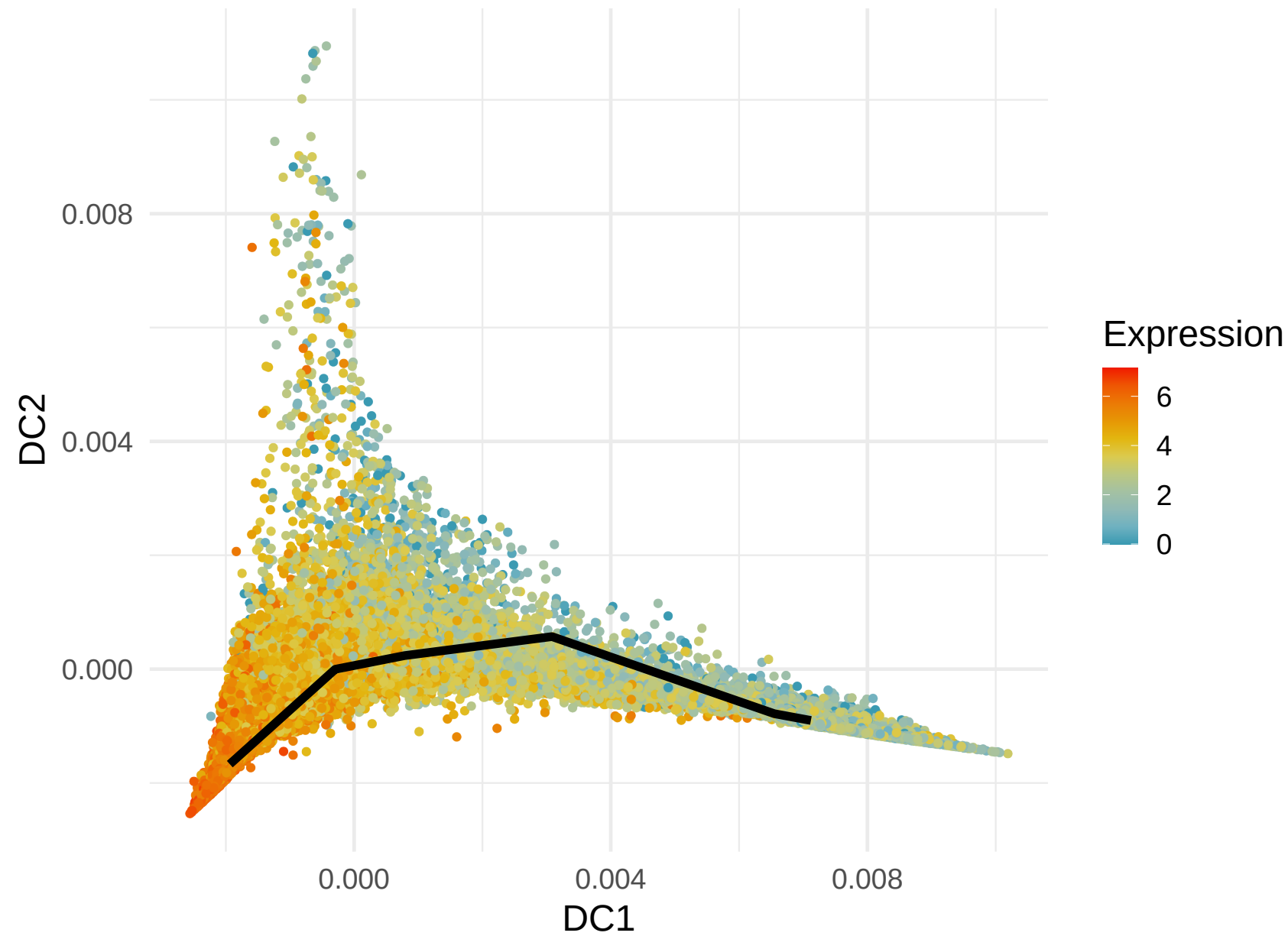
S100A9 Expression along Lineage 3 ( R = -0.611 )
