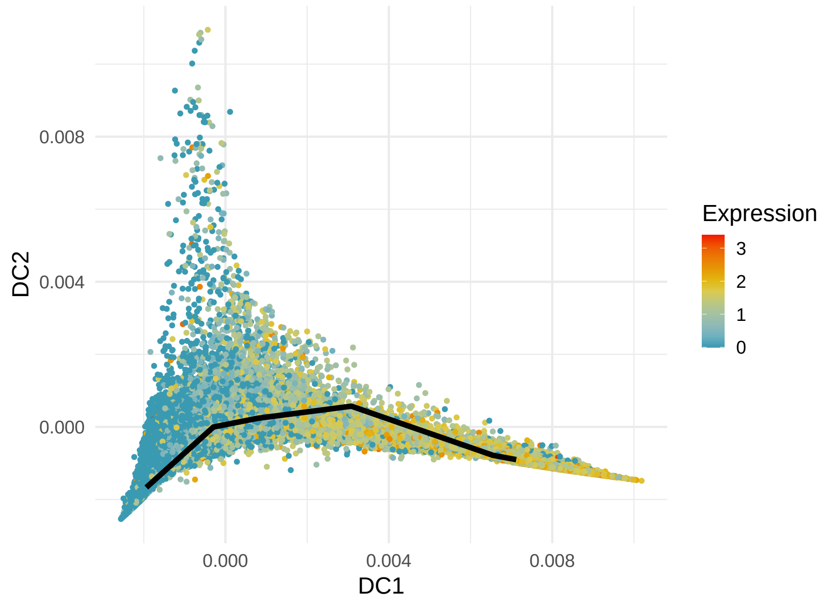
TCF7L2 Expression along Lineage 3 ( R = 0.571 )
