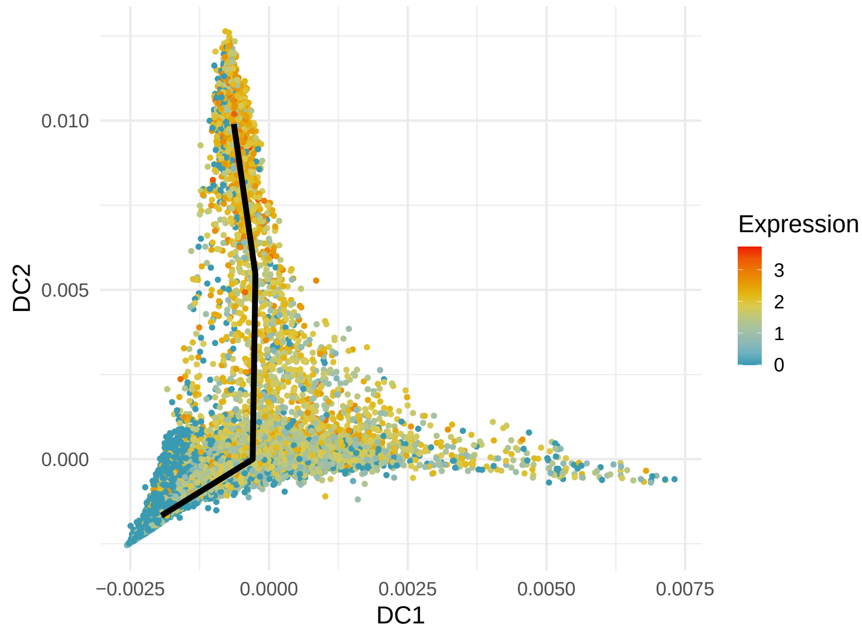
HLA-DMA Expression along Lineage 4 ( R = 0.322 )
