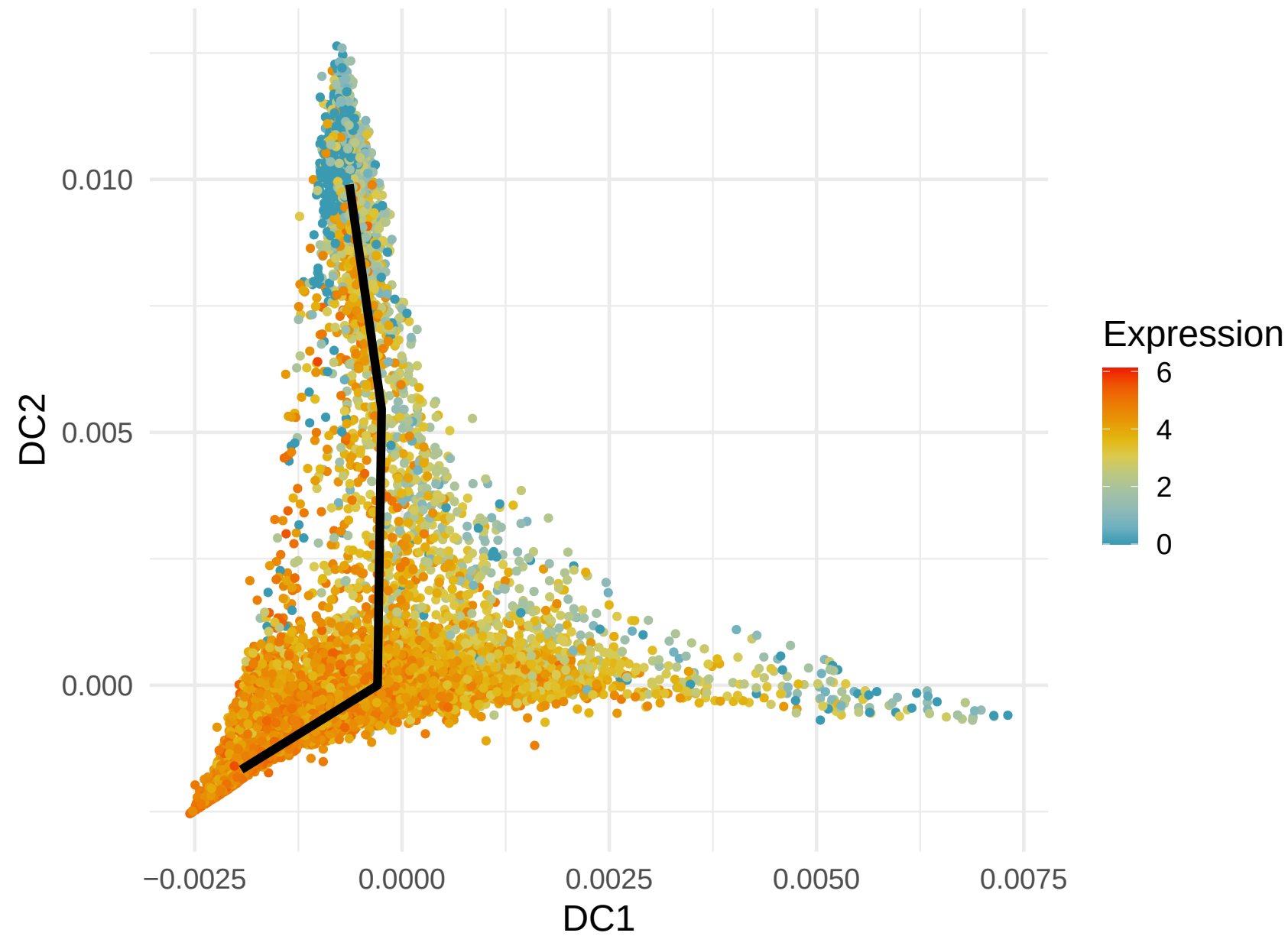
LYZ Expression along Lineage 4 ( R = -0.304 )
