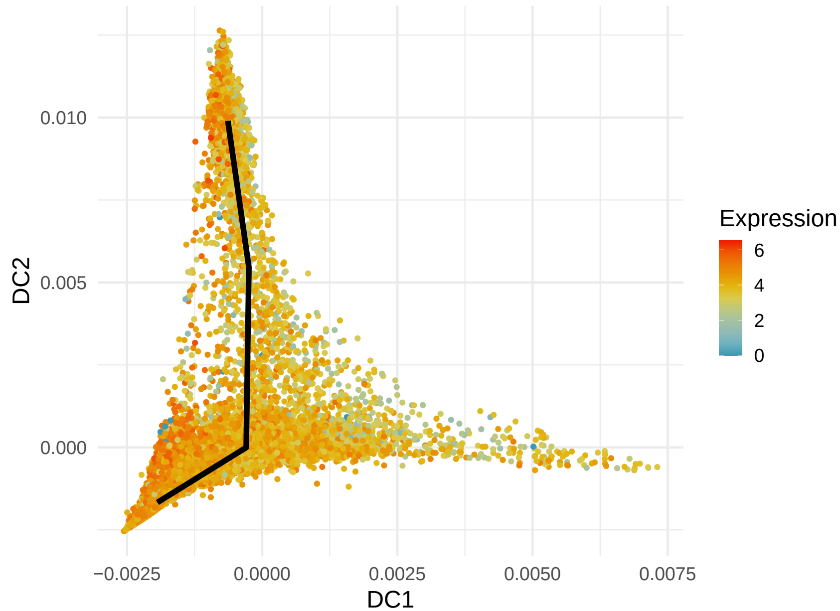
MT-CO3 Expression along Lineage 4 ( R = -0.28 )
