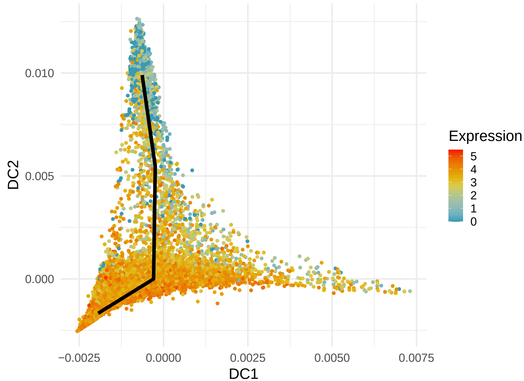
S100A6 Expression along Lineage 4 ( R = -0.311 )
