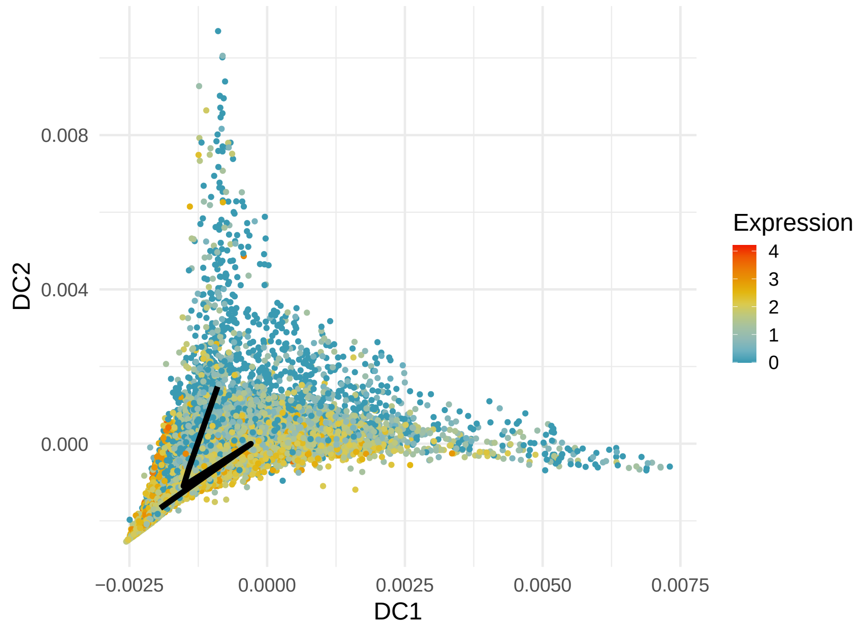
RIPOR2 Expression along Lineage 5 ( R = -0.213 )
