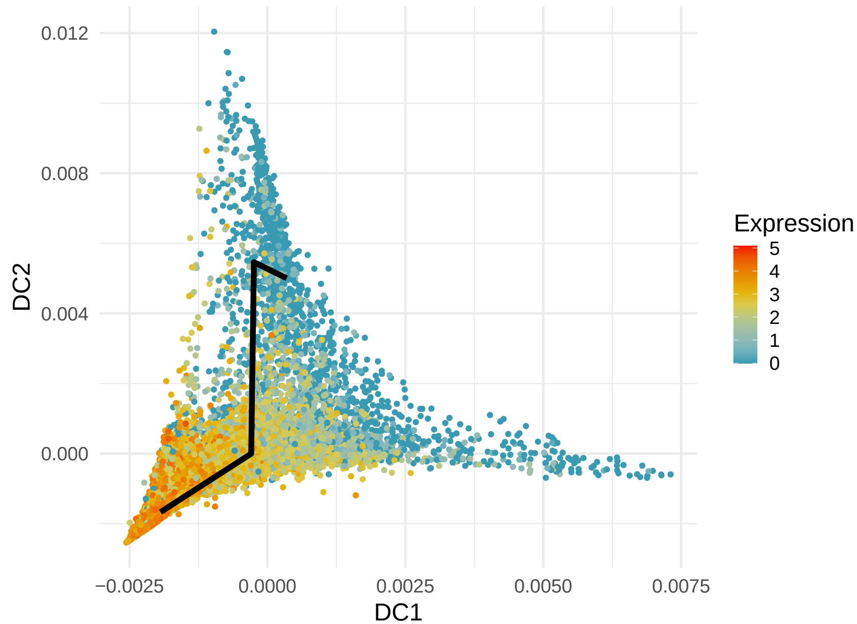
VCAN Expression along Lineage 6 ( R = -0.396 )
