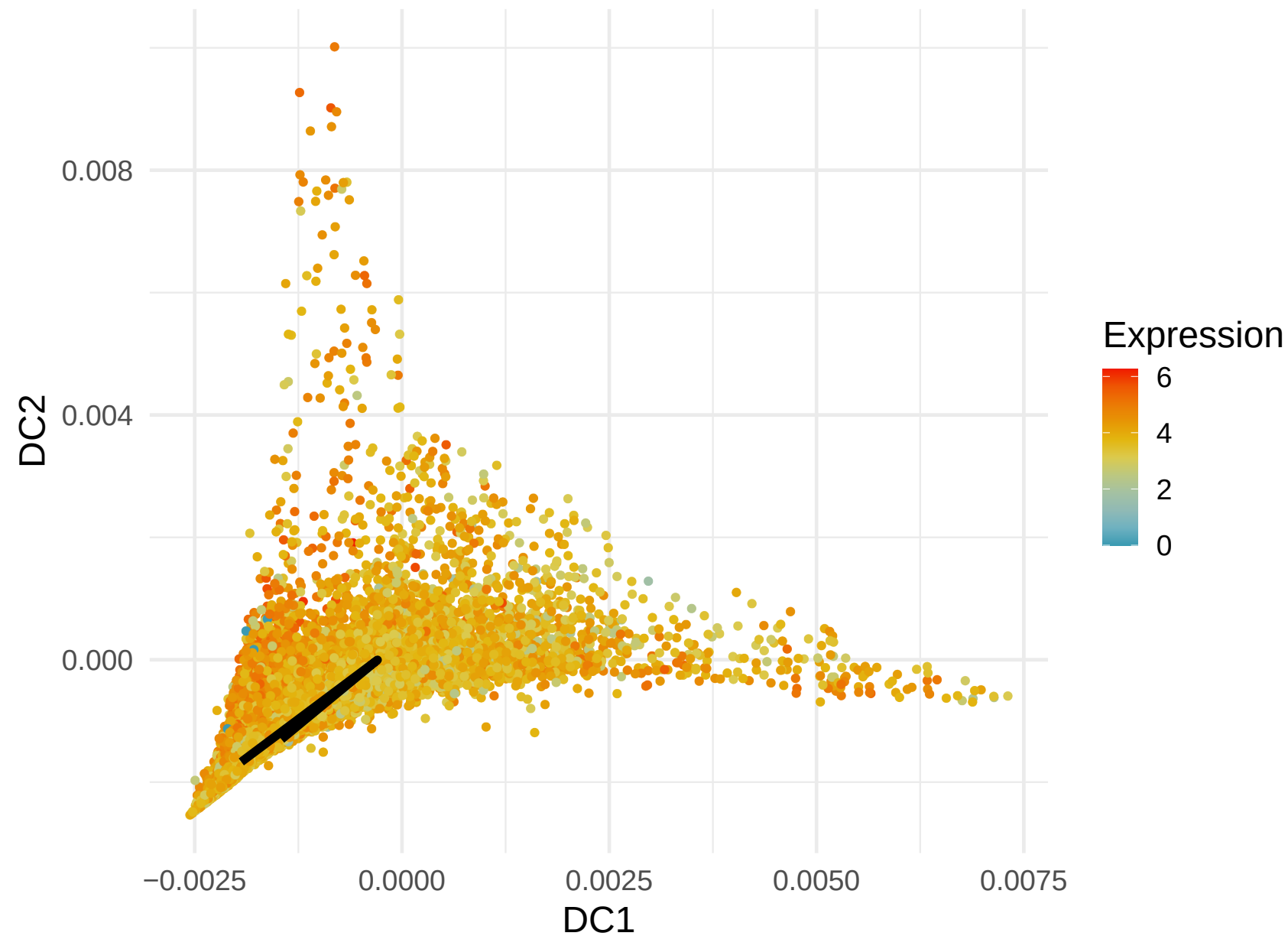
MT-ND4 Expression along Lineage 8 ( R = -0.205 )
