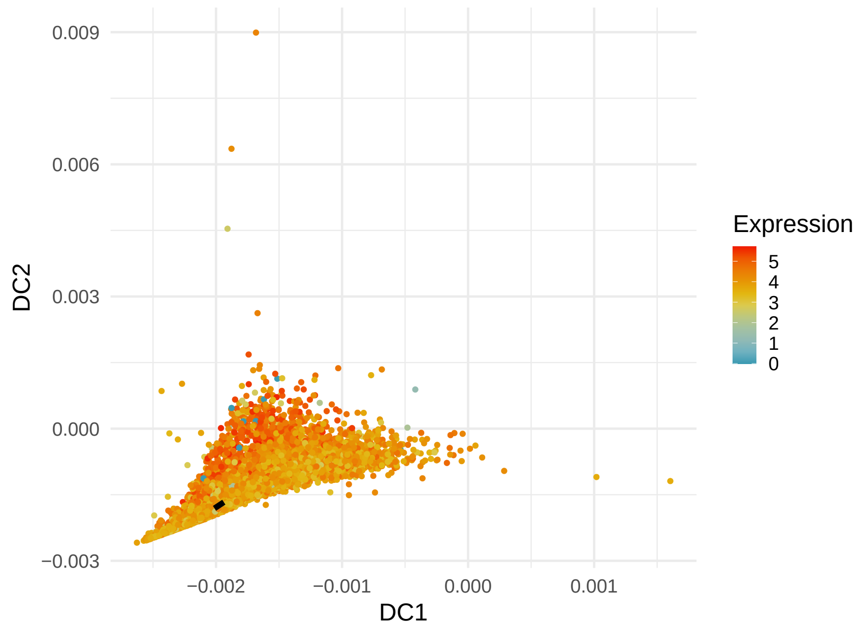
MT-ND1 Expression along Lineage 9 ( R = -0.245 )
