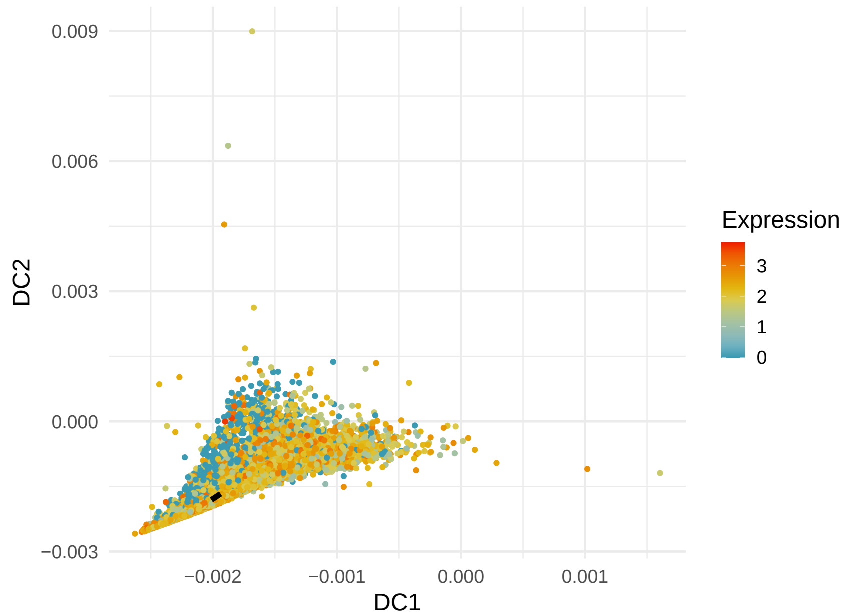
RPL10A Expression along Lineage 9 ( R = 0.437 )
