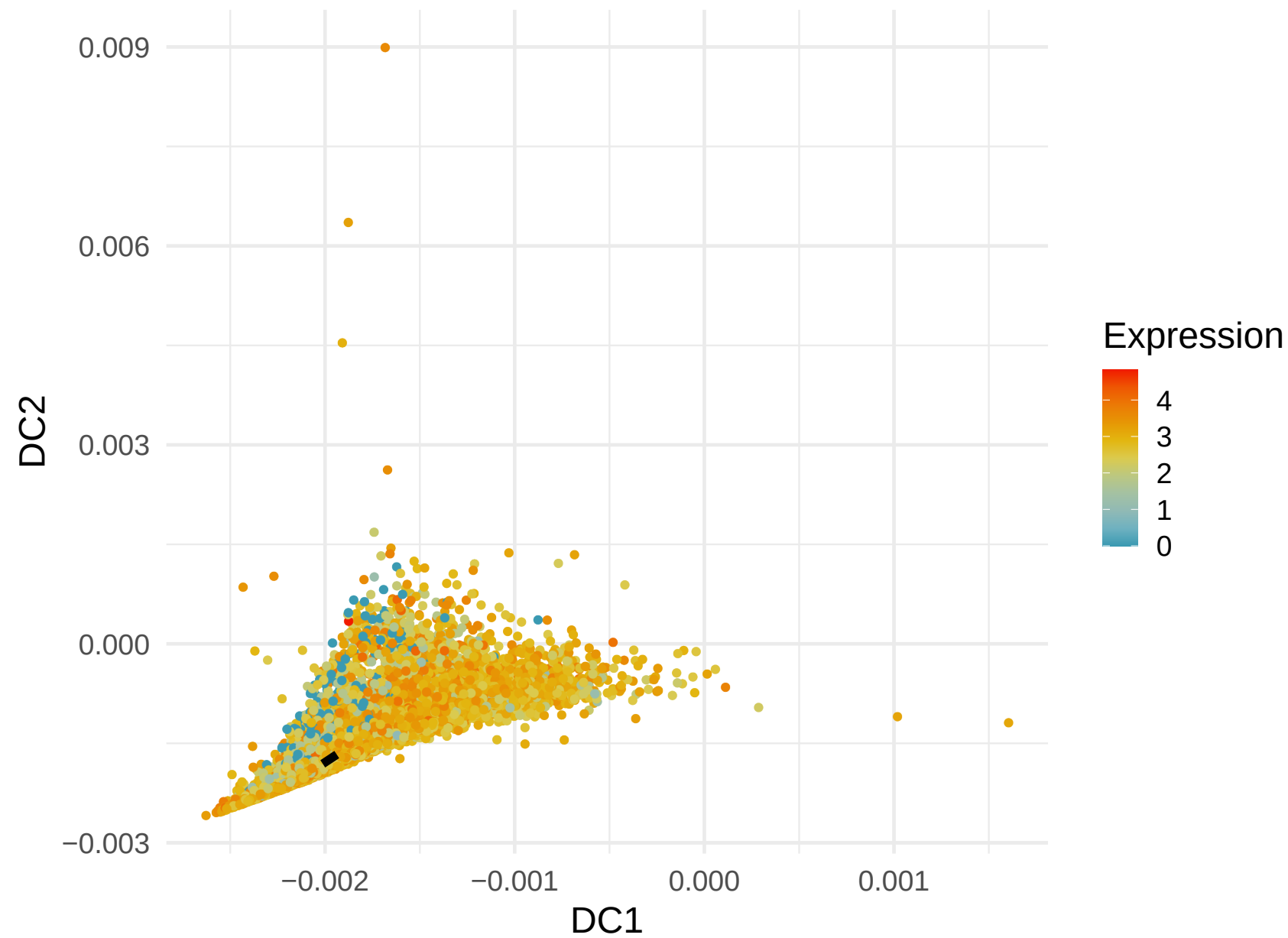
RPS2 Expression along Lineage 9 ( R = 0.482 )
