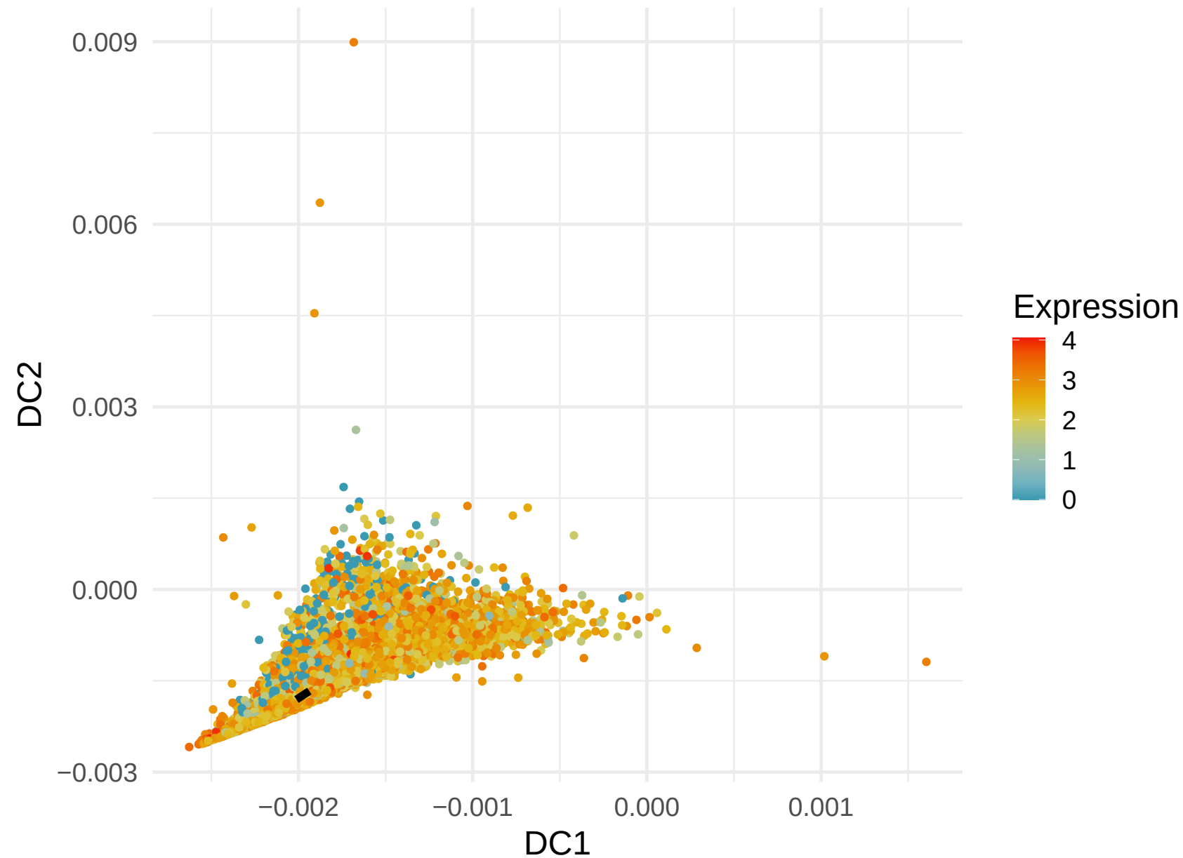
RPS4X Expression along Lineage 9 ( R = 0.423 )
