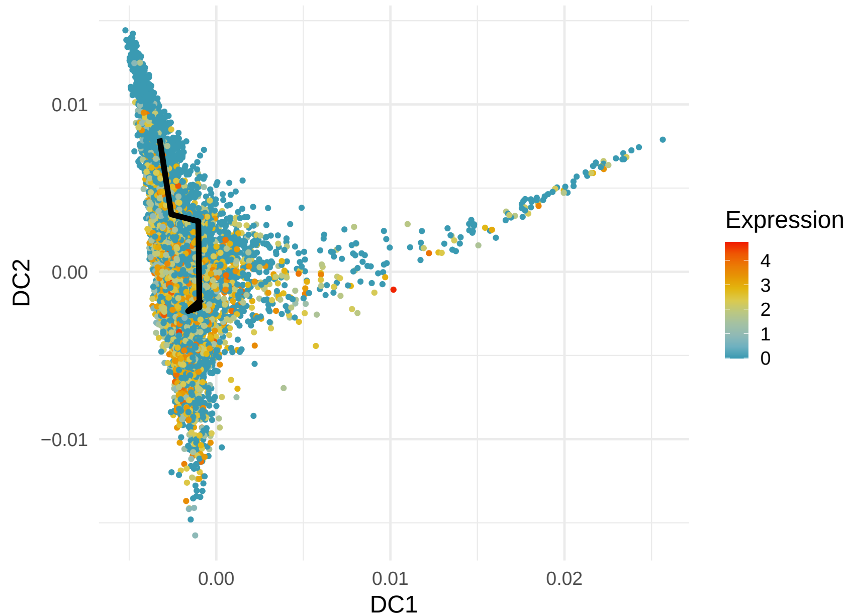
KLRB1 Expression along Lineage 1 ( R= 0.335 )
