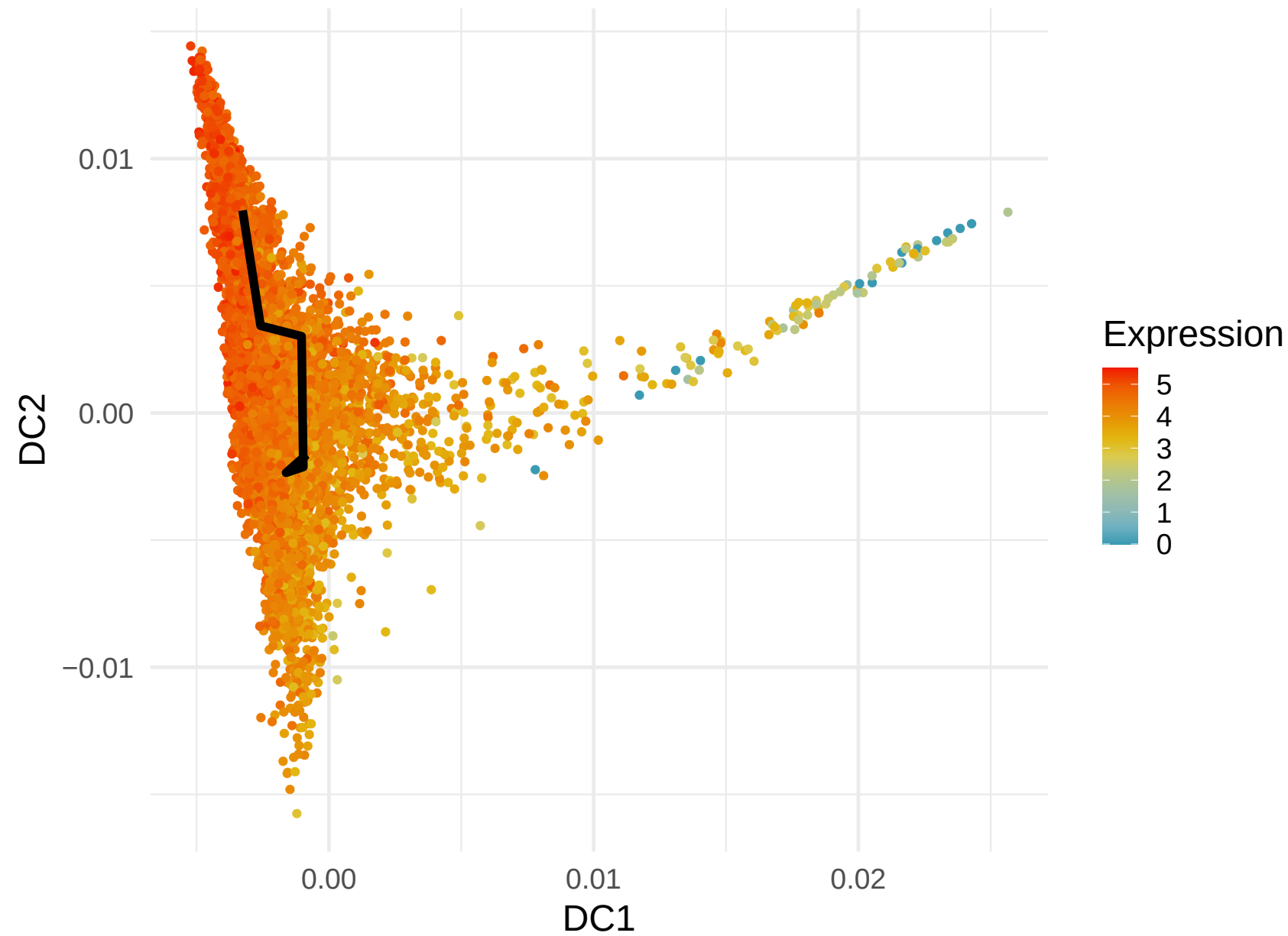
RPS12 Expression along Lineage 1 ( R = -0.337 )
