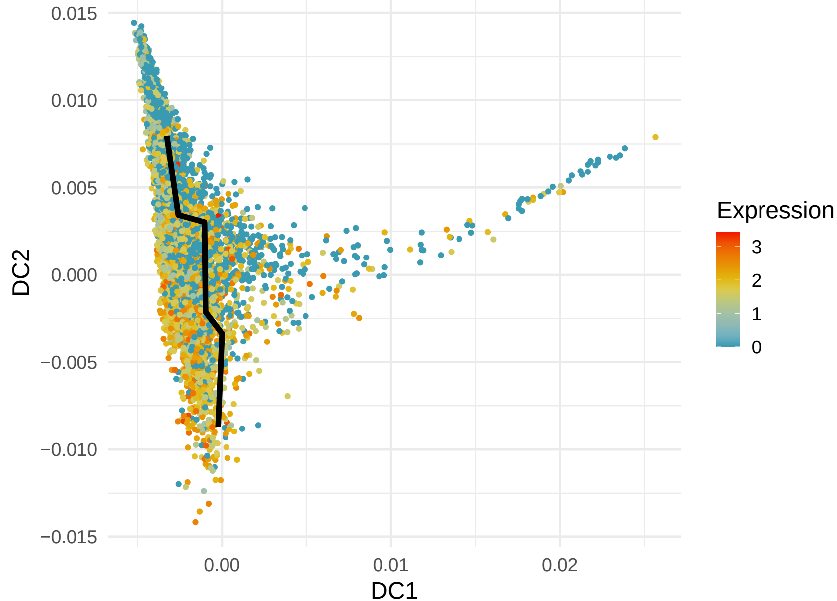
CLIC1 Expression along Lineage 2 ( R= 0.253 )
