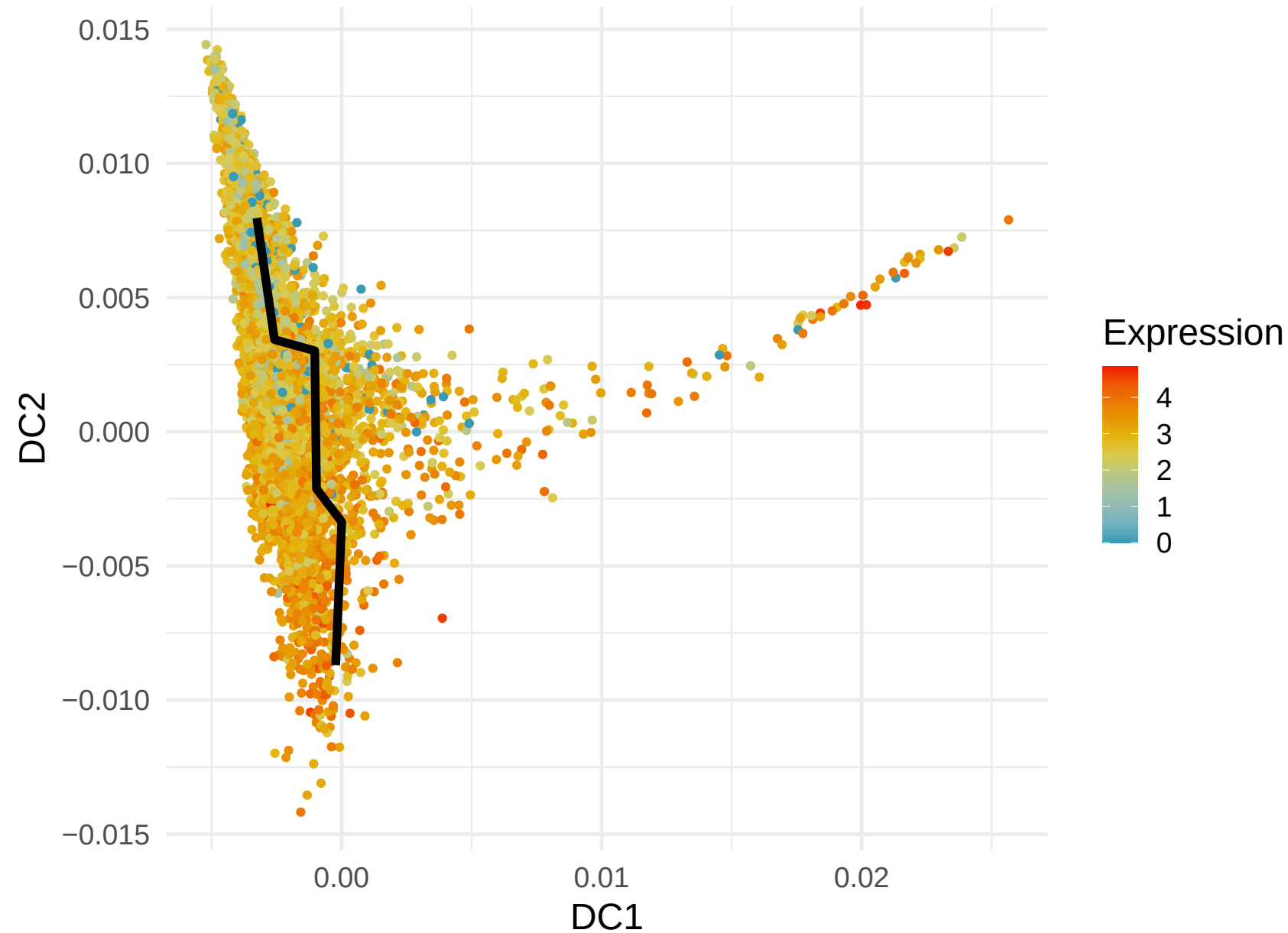
HLA-A Expression along Lineage 2 ( R = 0.272 )
