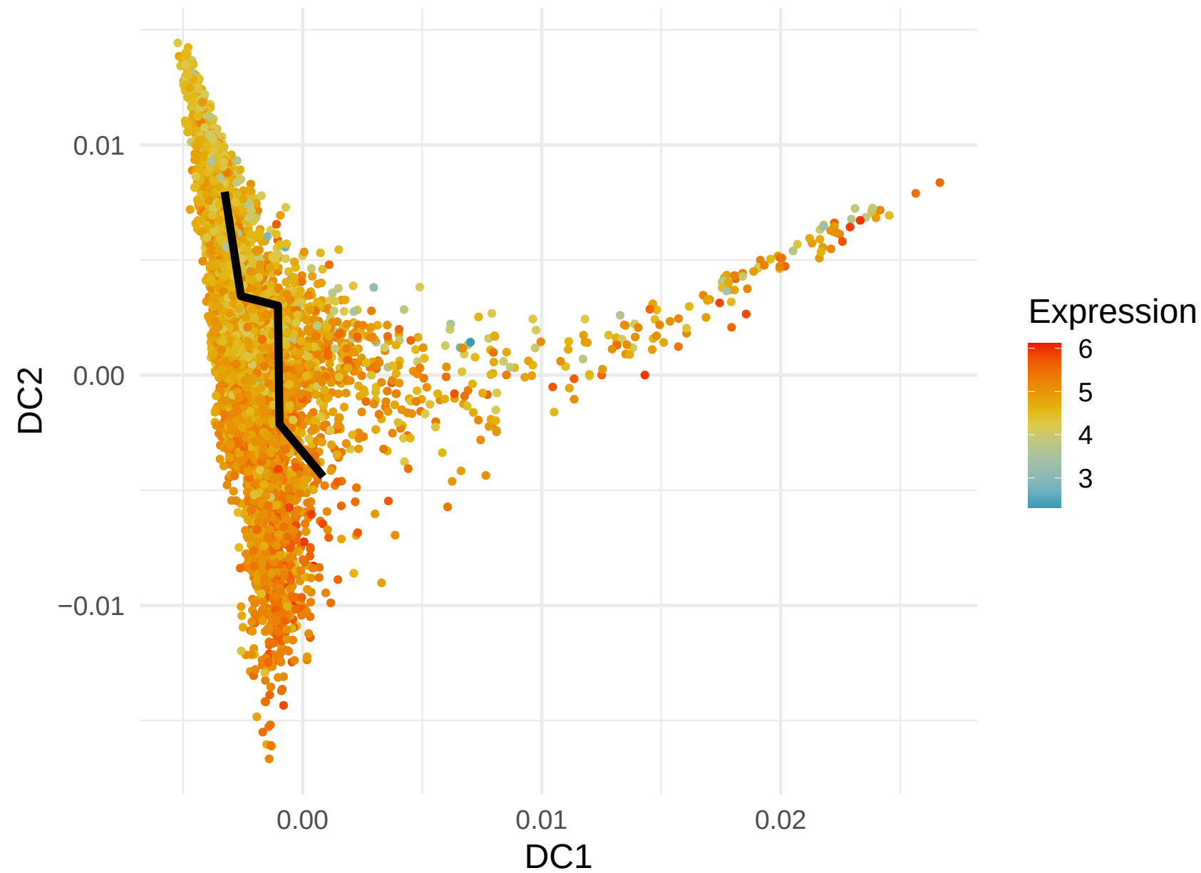
B2M Expression along Lineage 3 ( R = 0.456 )
