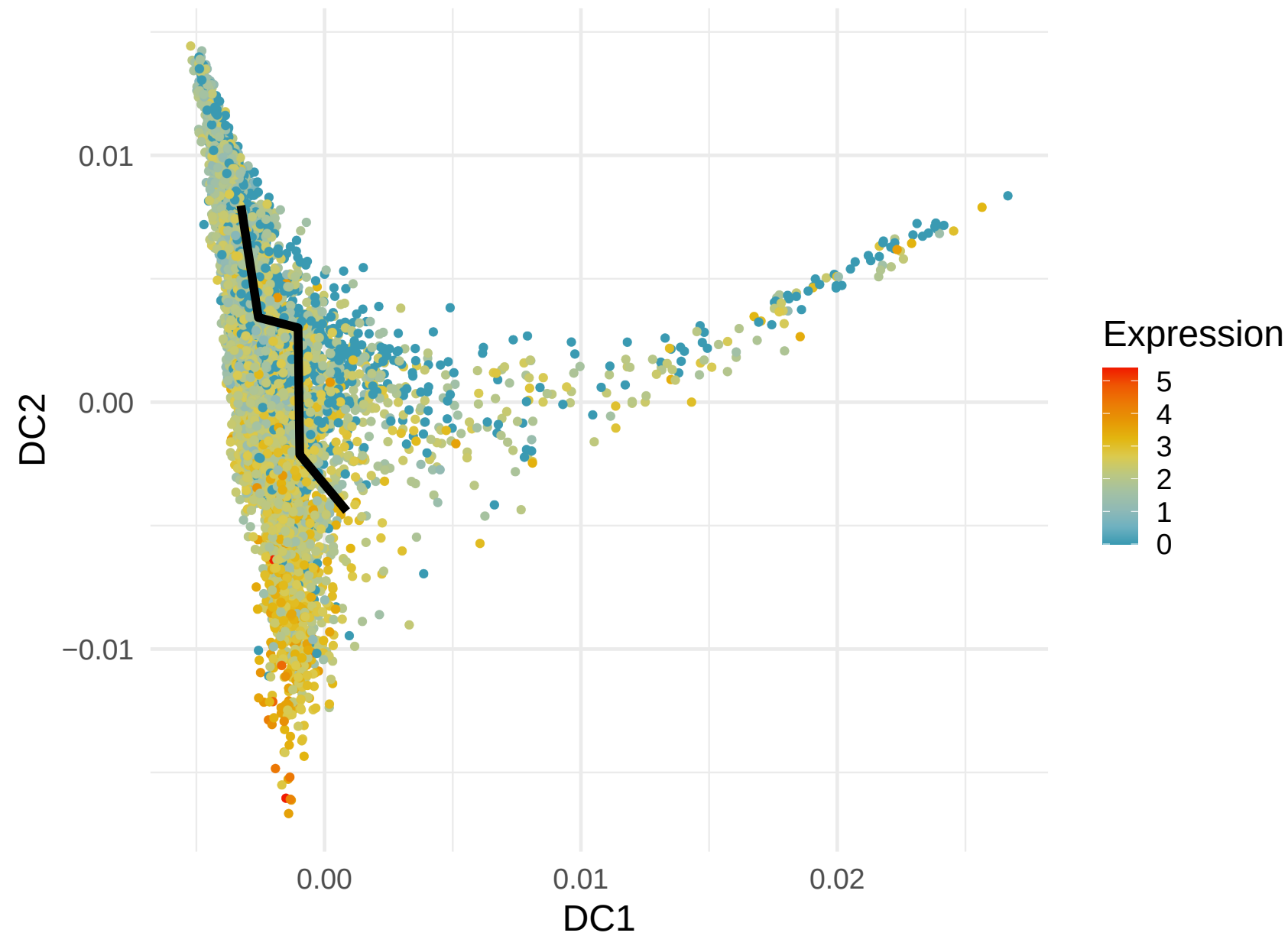
GAPDH Expression along Lineage 3 ( R = 0.348 )
