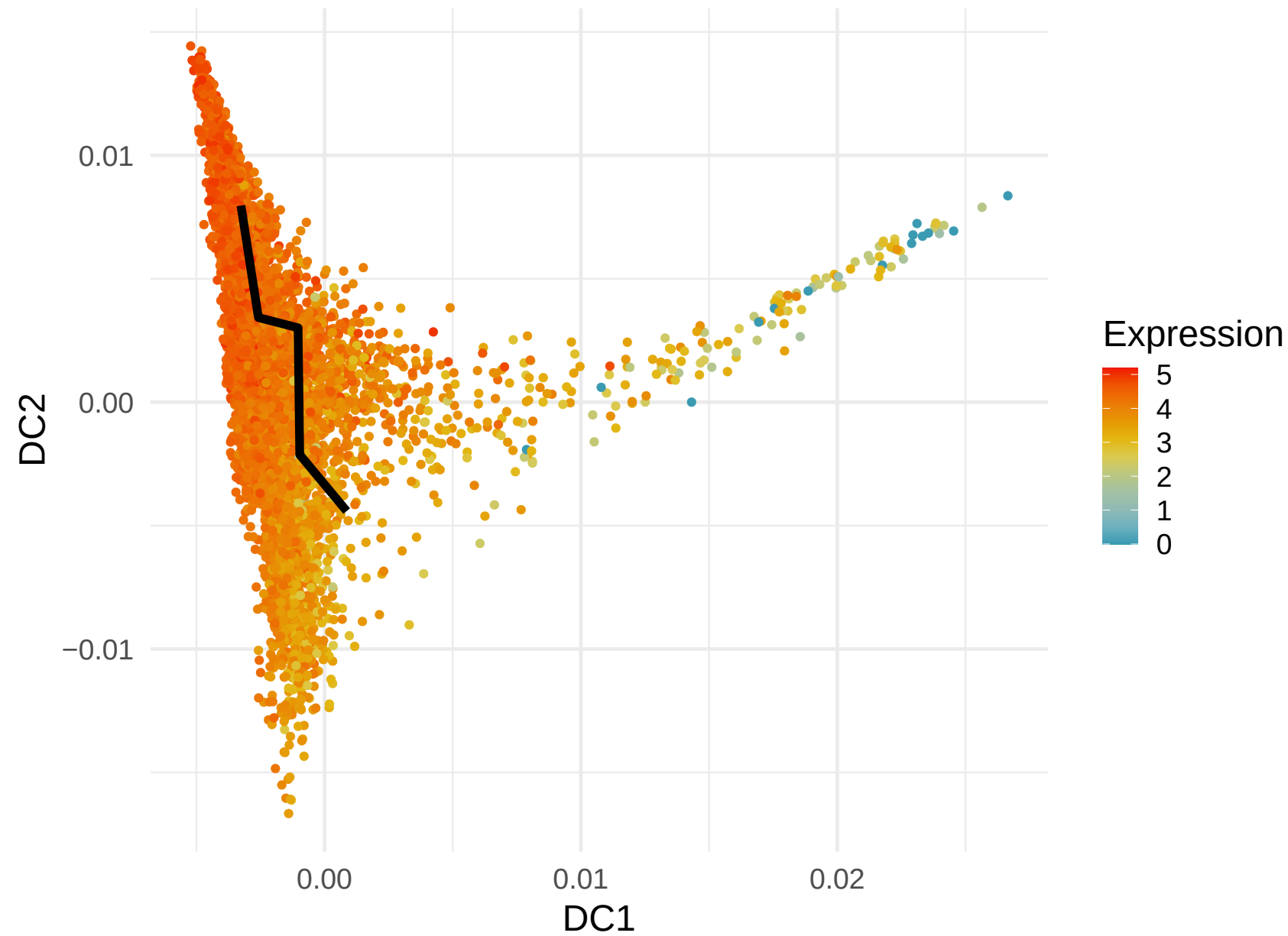
RPL32 Expression along Lineage 3 ( R = -0.459 )
