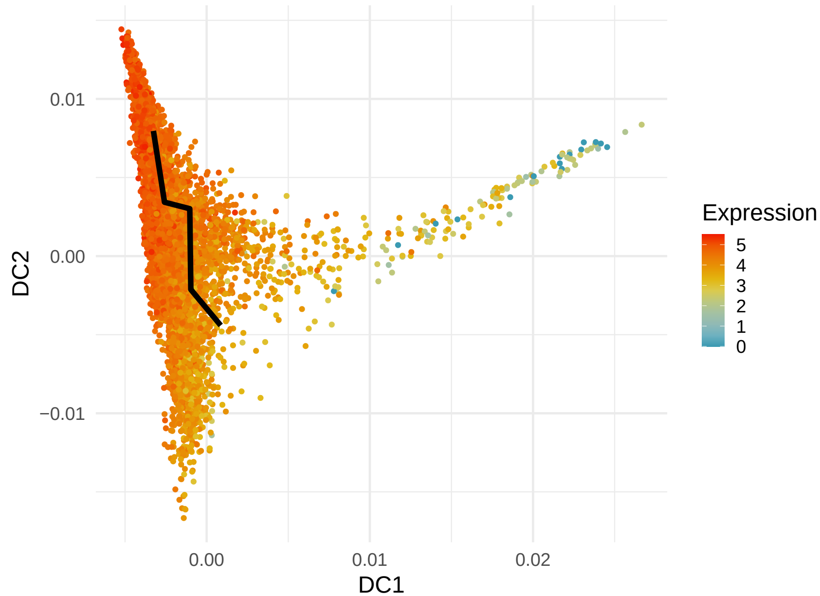
RPS12 Expression along Lineage 3 ( R = -0.443 )
