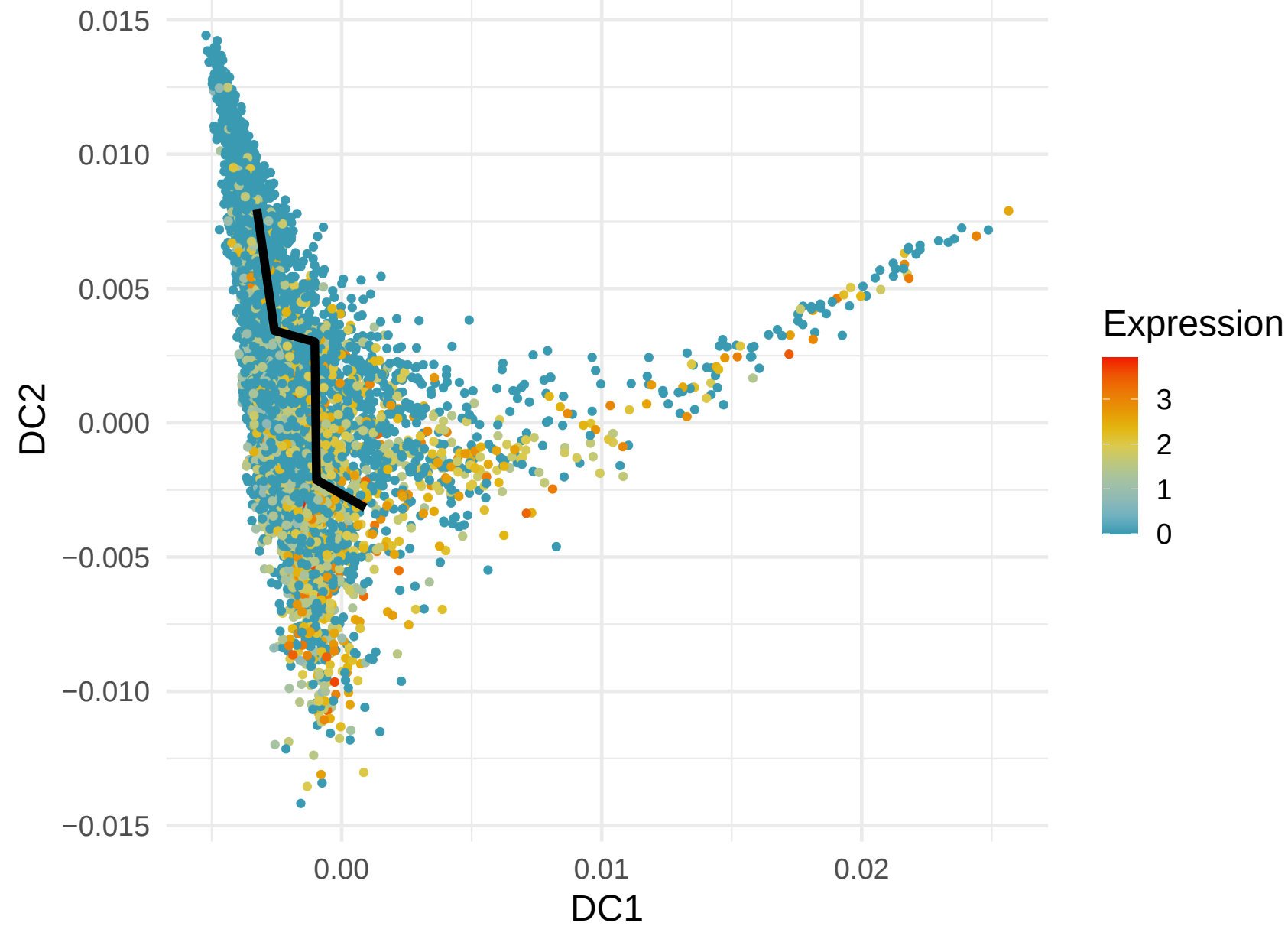
MAF Expression along Lineage 4 ( R = 0.262 )
