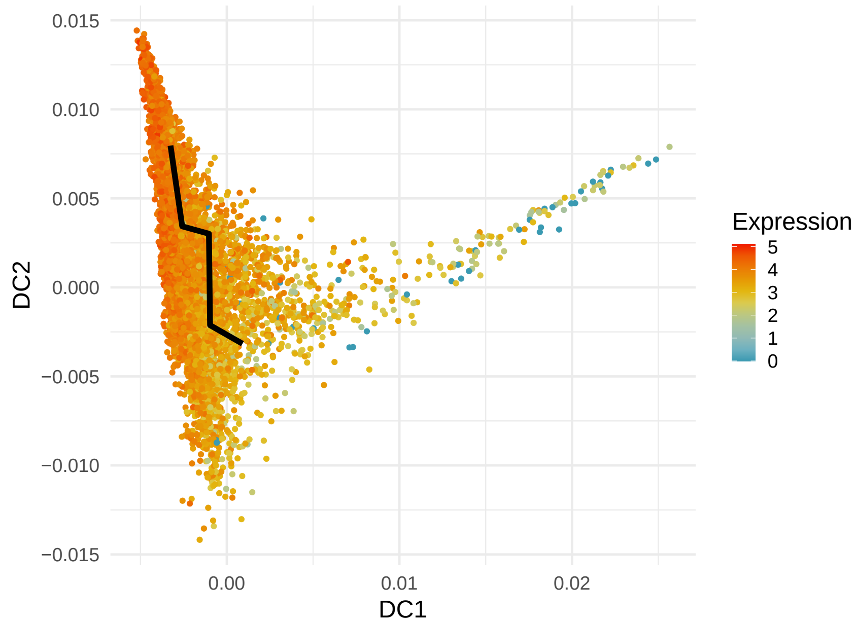
RPS8 Expression along Lineage 4 ( R = -0.468 )
