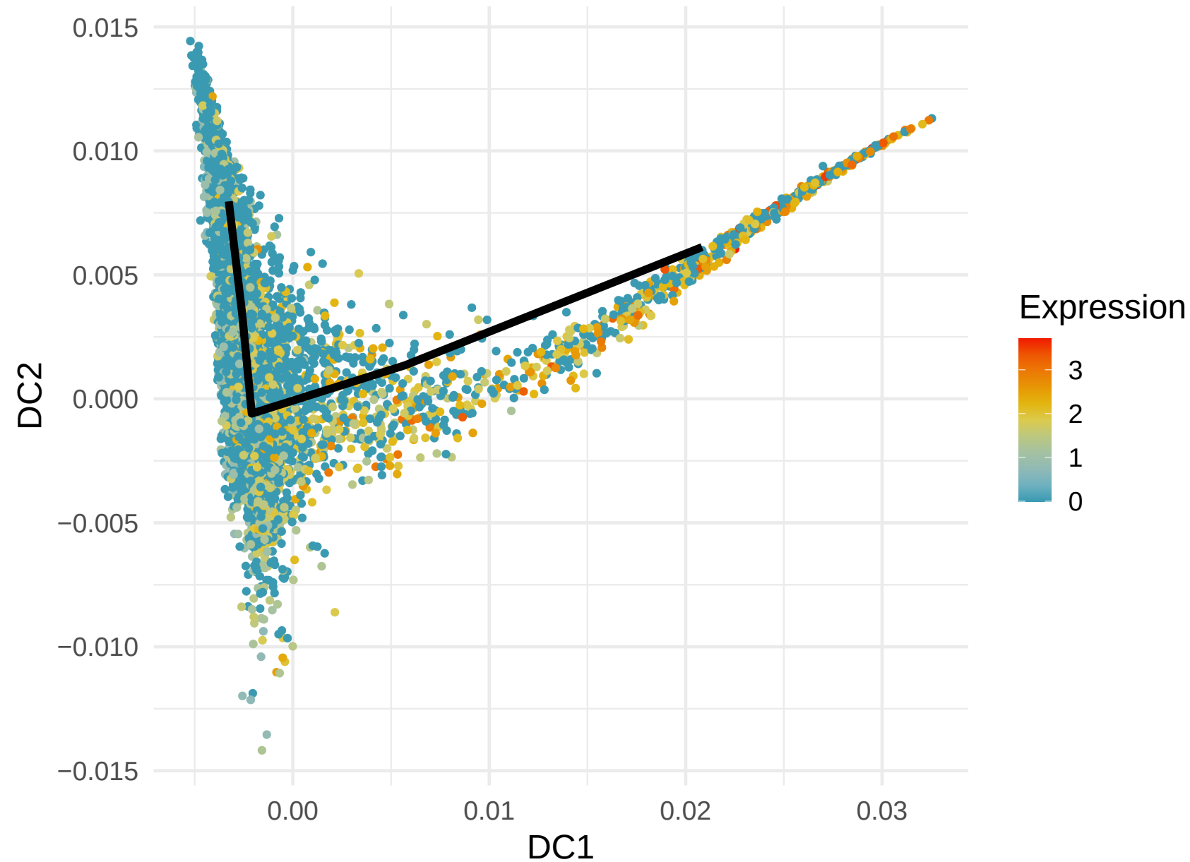
MACF1 Expression along Lineage 5 ( R= 0.251 )
