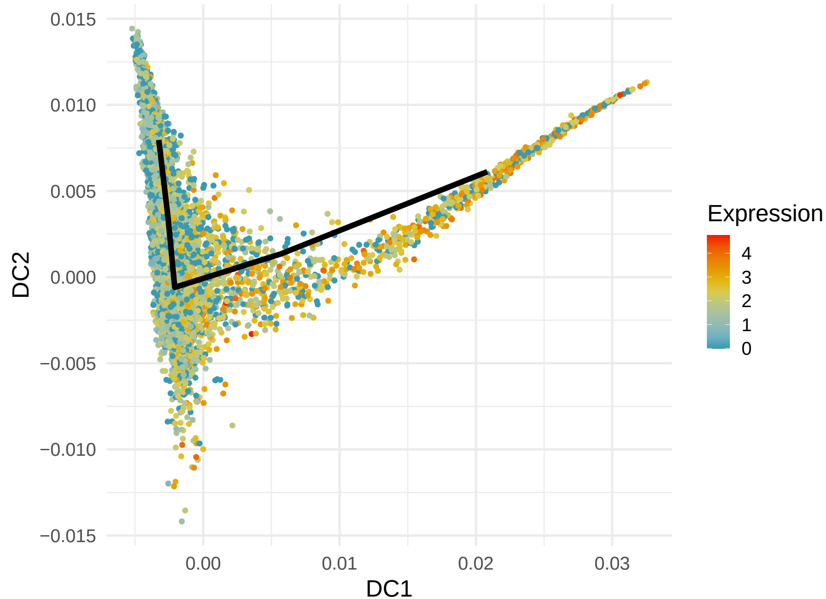
NEAT1 Expression along Lineage 5 ( R = 0.221 )
