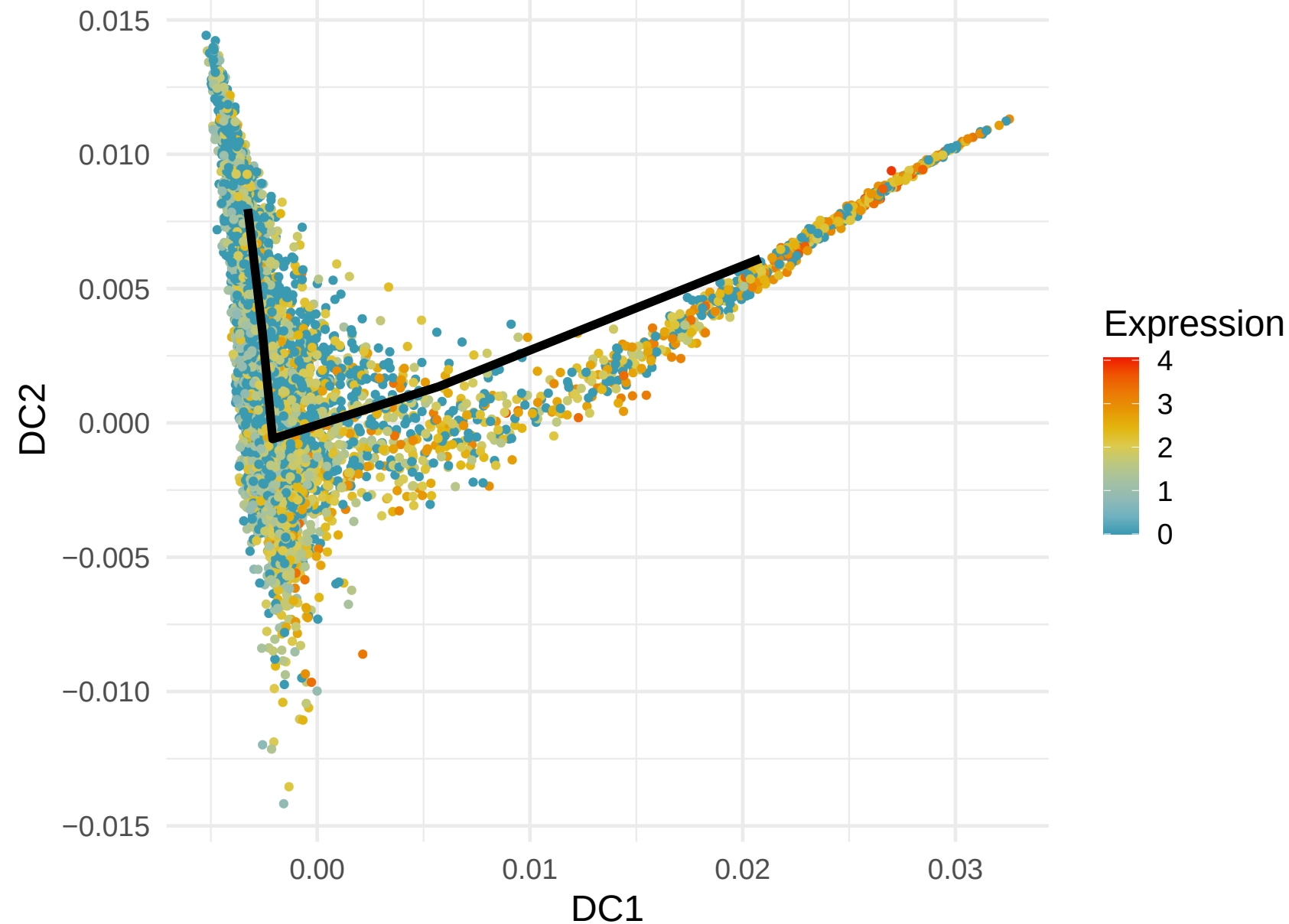
RNF213 Expression along Lineage 5 ( R = 0.221 )
