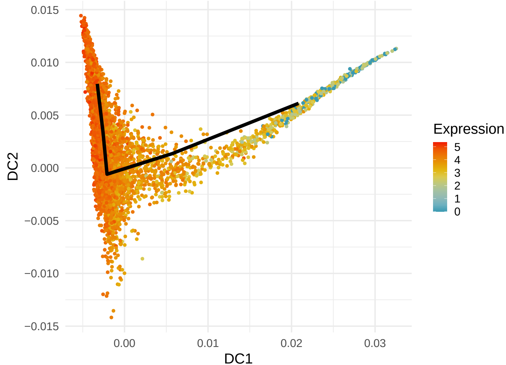
RPS18 Expression along Lineage 5 ( R = -0.705 )
