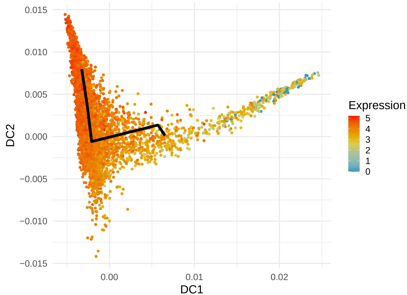
RPL32 Expression along Lineage 6 ( R = -0.483 )
