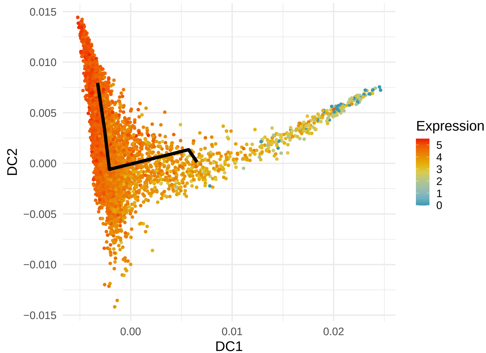
RPS12 Expression along Lineage 6 ( R = -0.503 )
