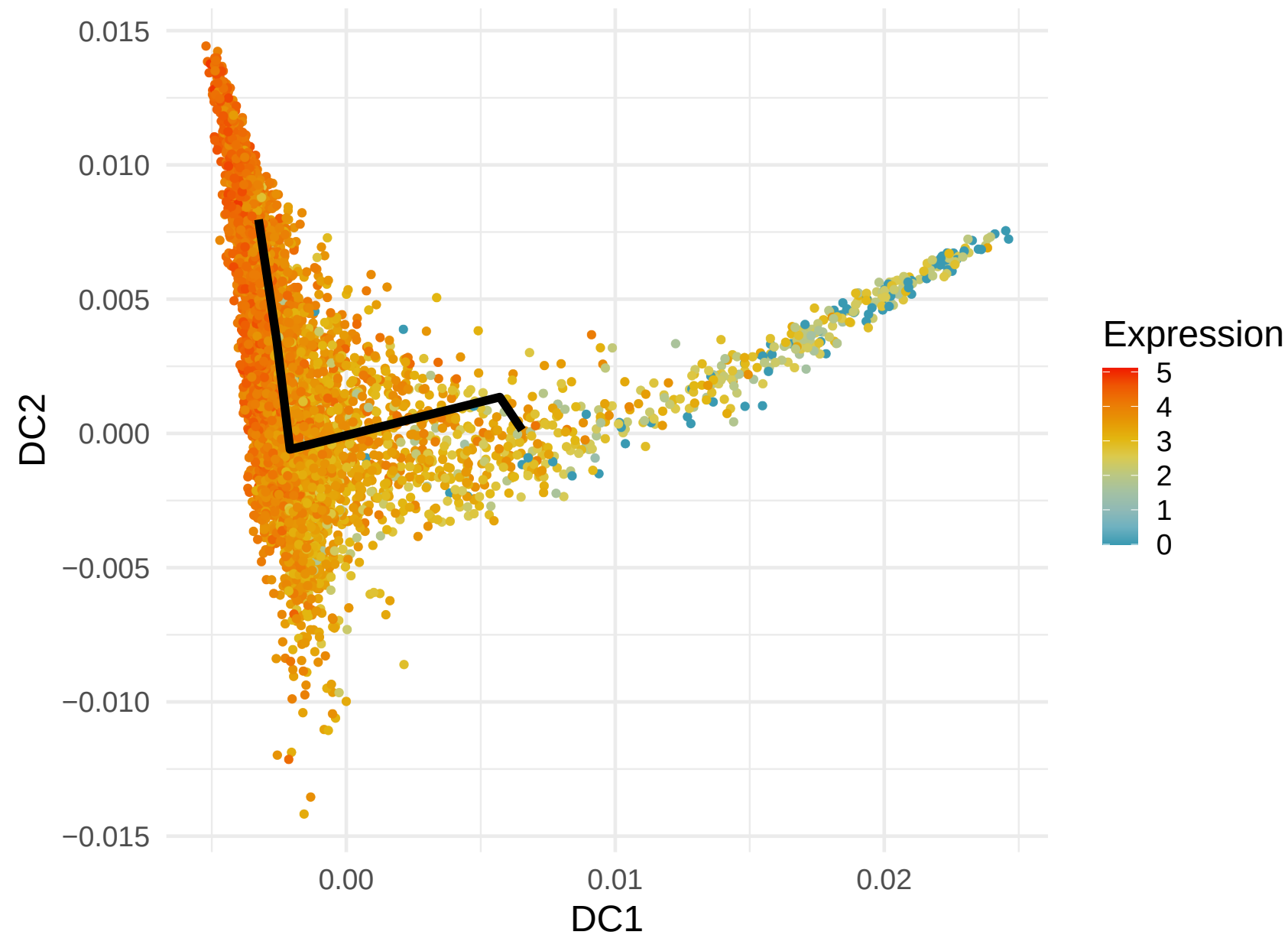
RPS8 Expression along Lineage 6 ( R = -0.458 )
