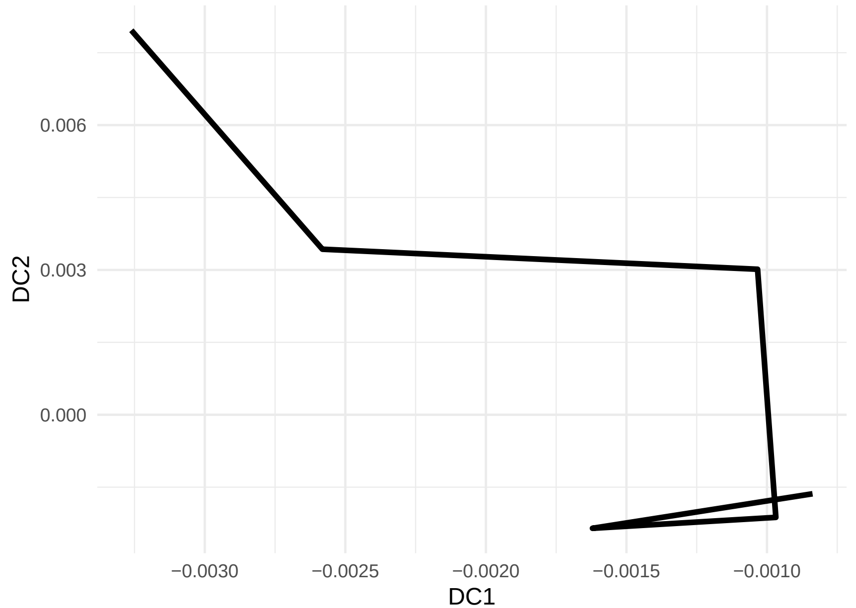
AC136612.1 Expression along Lineage 1 (R= NA)
