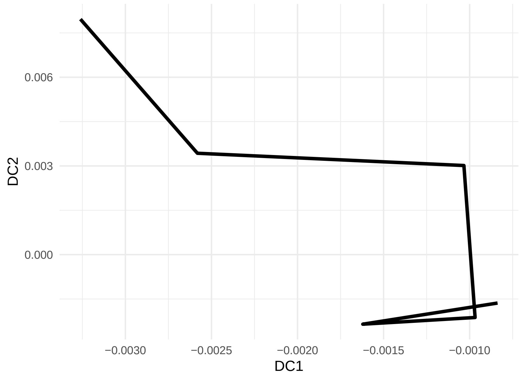
AL627309.2 Expression along Lineage 1 (R= NA)
