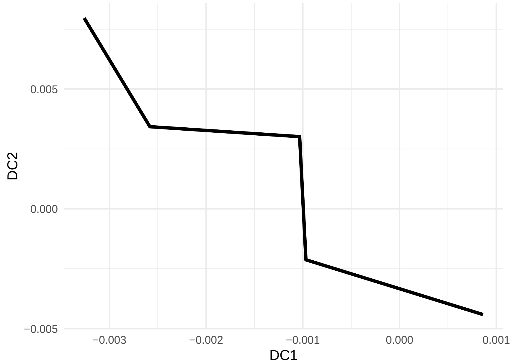
MIR1302-2HG Expression along Lineage 3 (R= NA)
