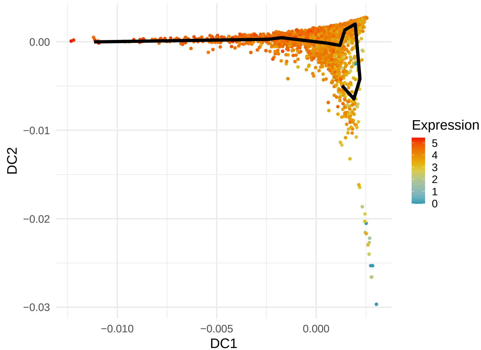
RPS12 Expression along Lineage 1 ( R = -0.345 )
