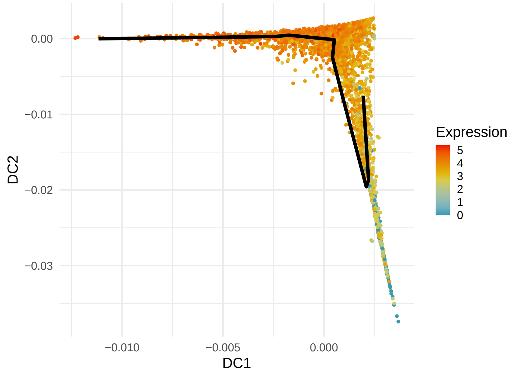
RPL10 Expression along Lineage 2 ( R = -0.498 )
