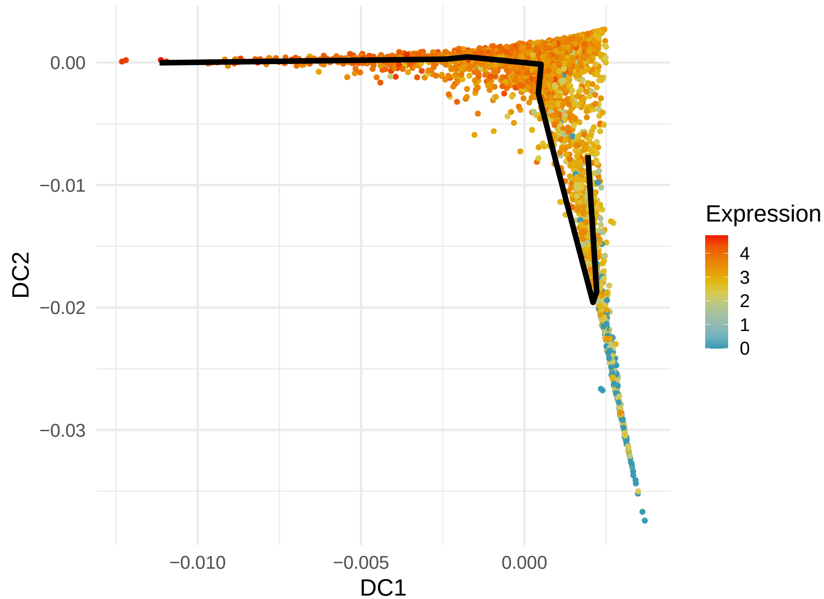
RPL19 Expression along Lineage 2 ( R = -0.503 )
