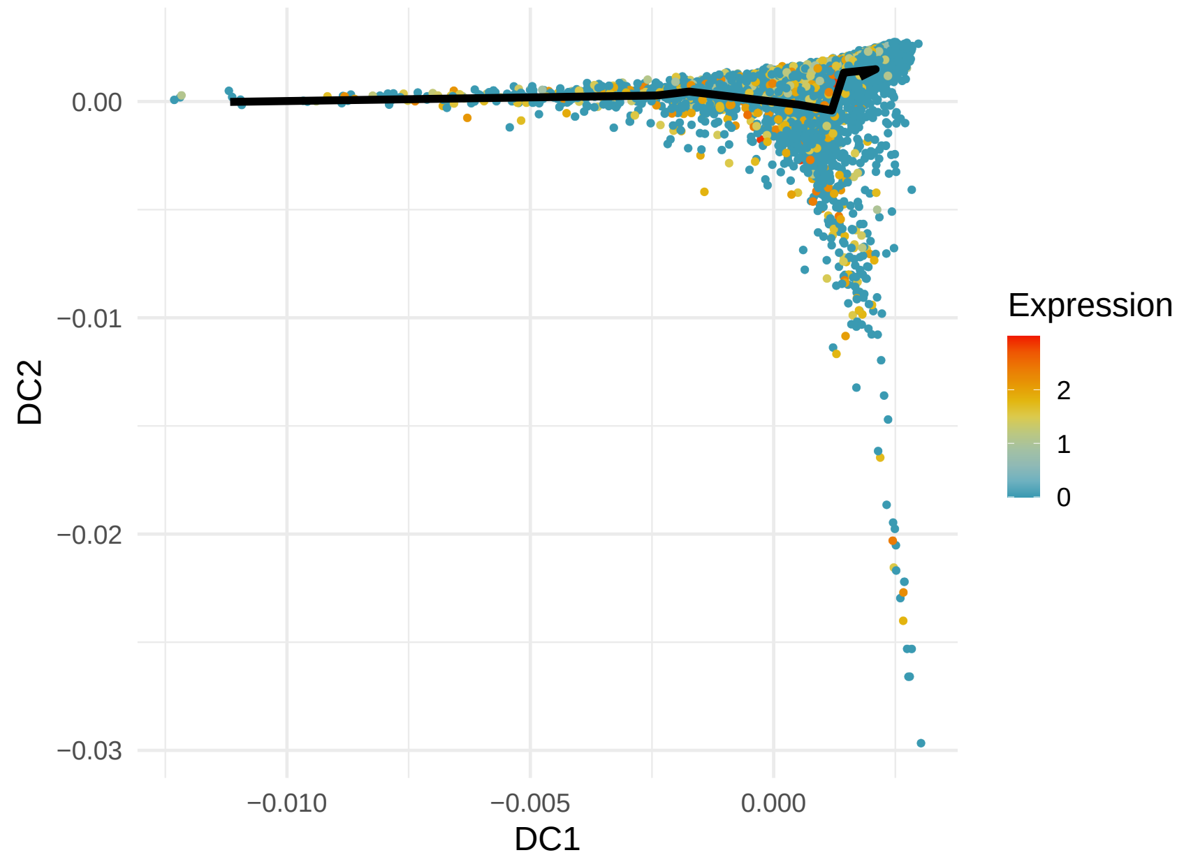
NCF1 Expression along Lineage 3 ( R = -0.231 )
