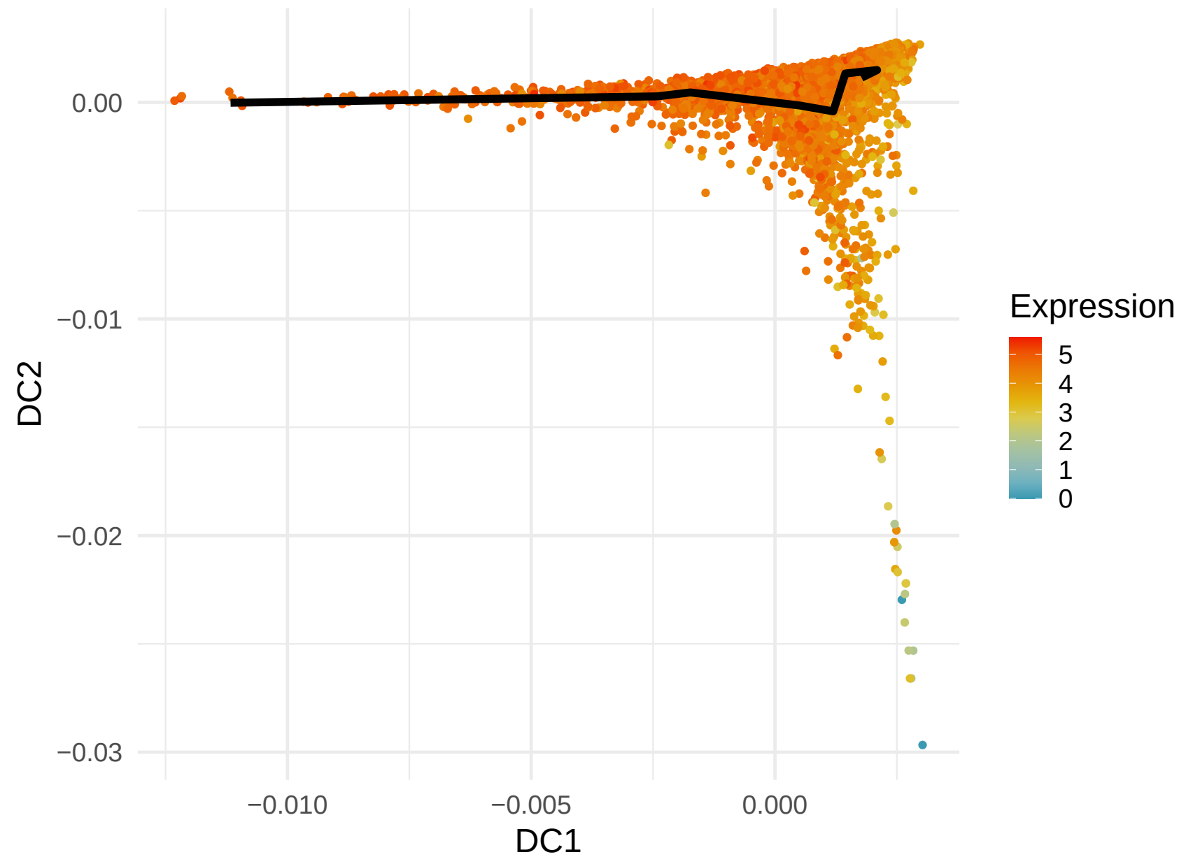
RPL41 Expression along Lineage 3 ( R = -0.254 )
