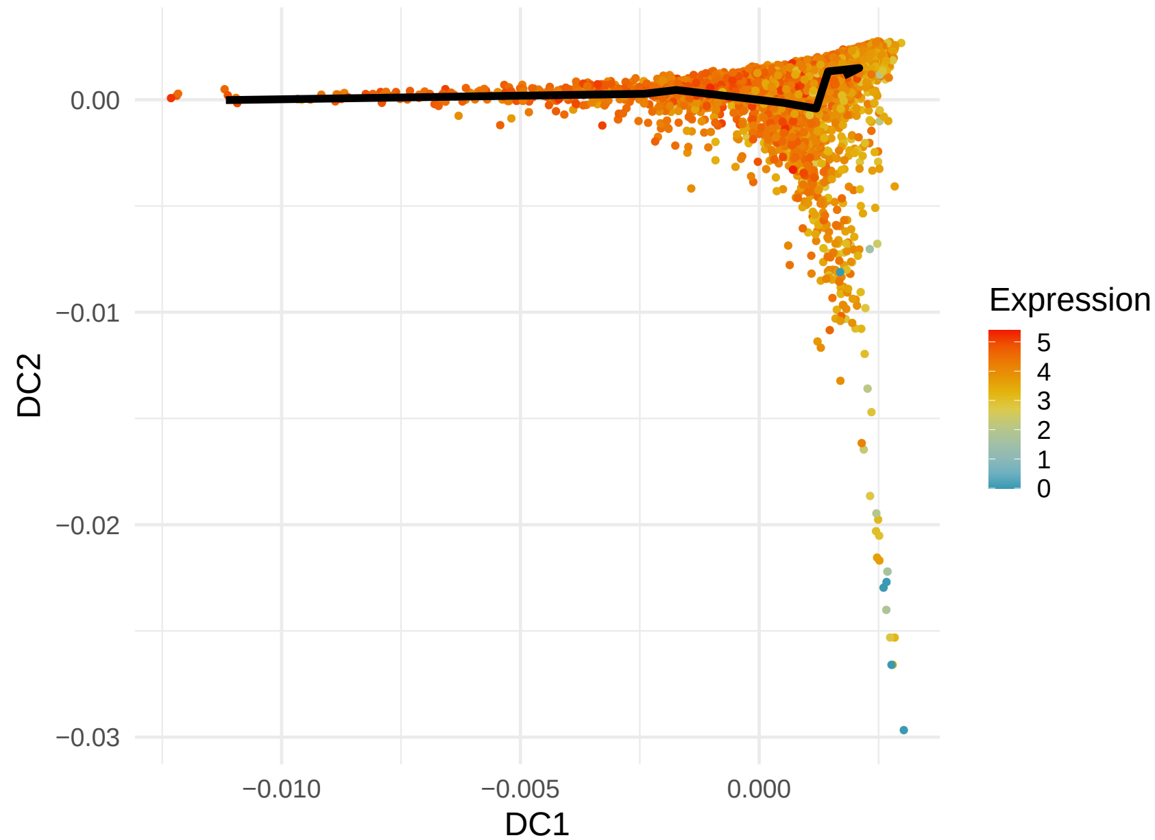
RPS29 Expression along Lineage 3 ( R = -0.304 )
