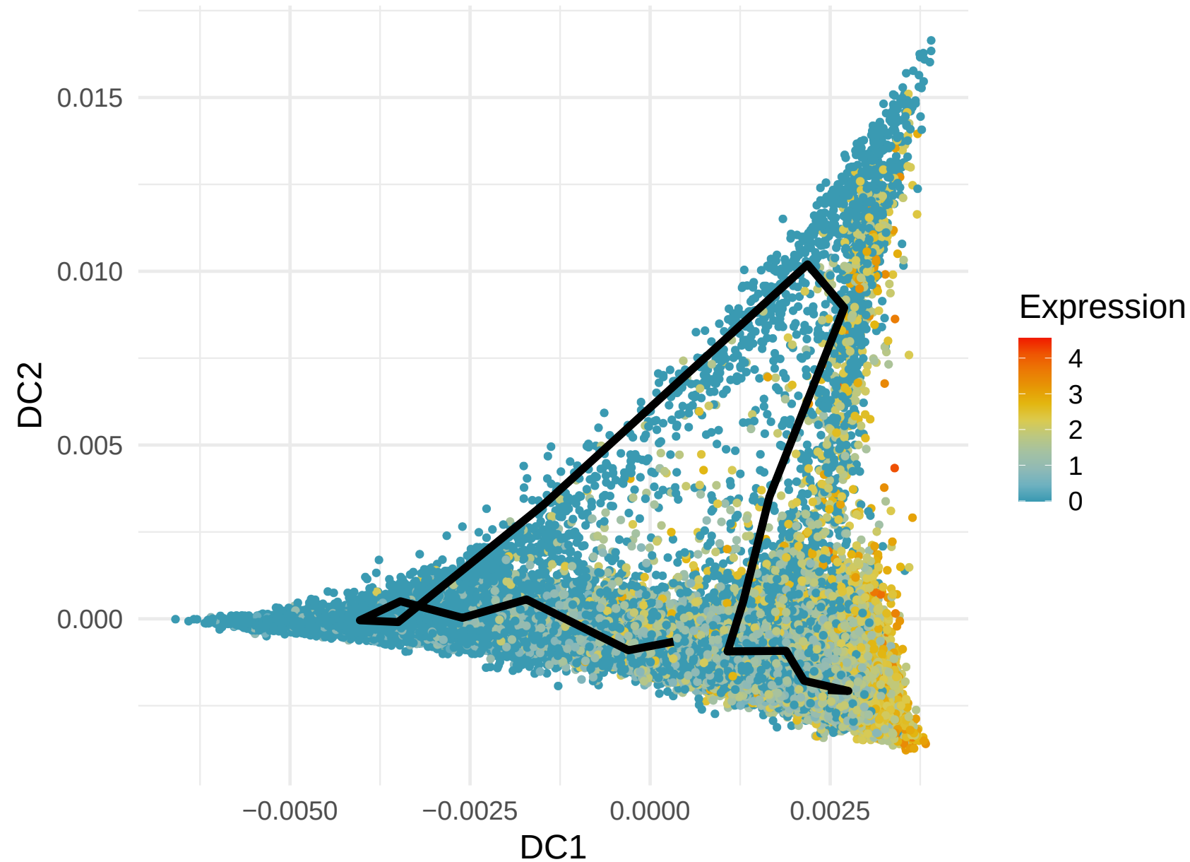
PRF1 Expression along Lineage 1 ( R = 0.523 )
