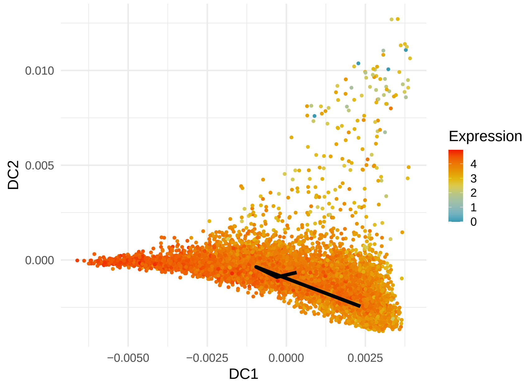
RPL30 Expression along Lineage 10 ( R = -0.316 )
