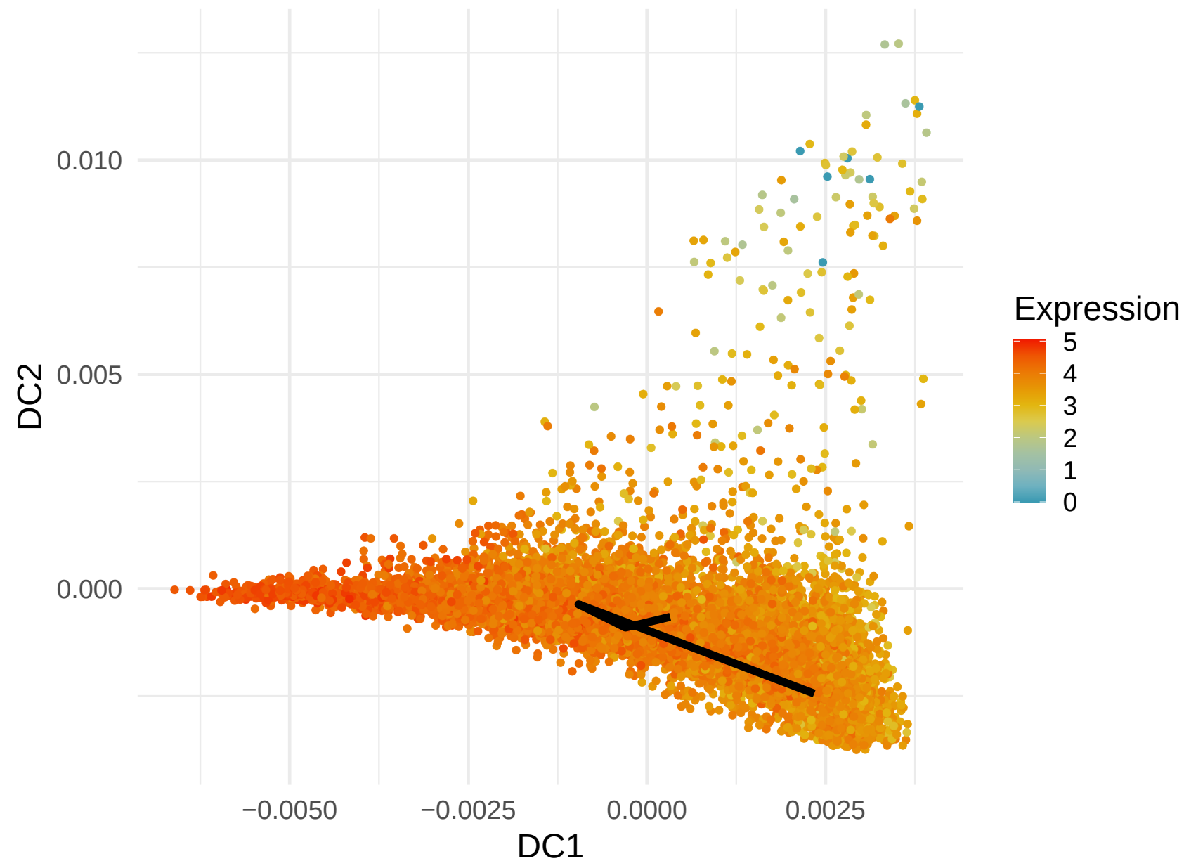
RPL32 Expression along Lineage 10 ( R = -0.29 )
