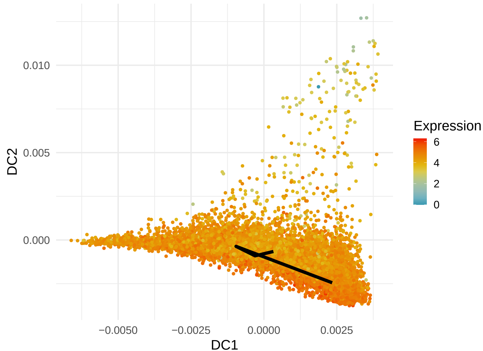
TMSB4X Expression along Lineage 10 ( R = 0.388 )
