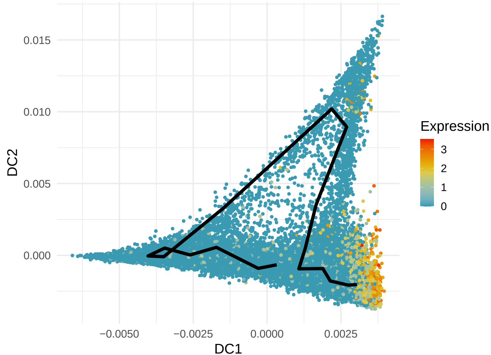
FCGR3A Expression along Lineage 2 ( R = 0.52 )
