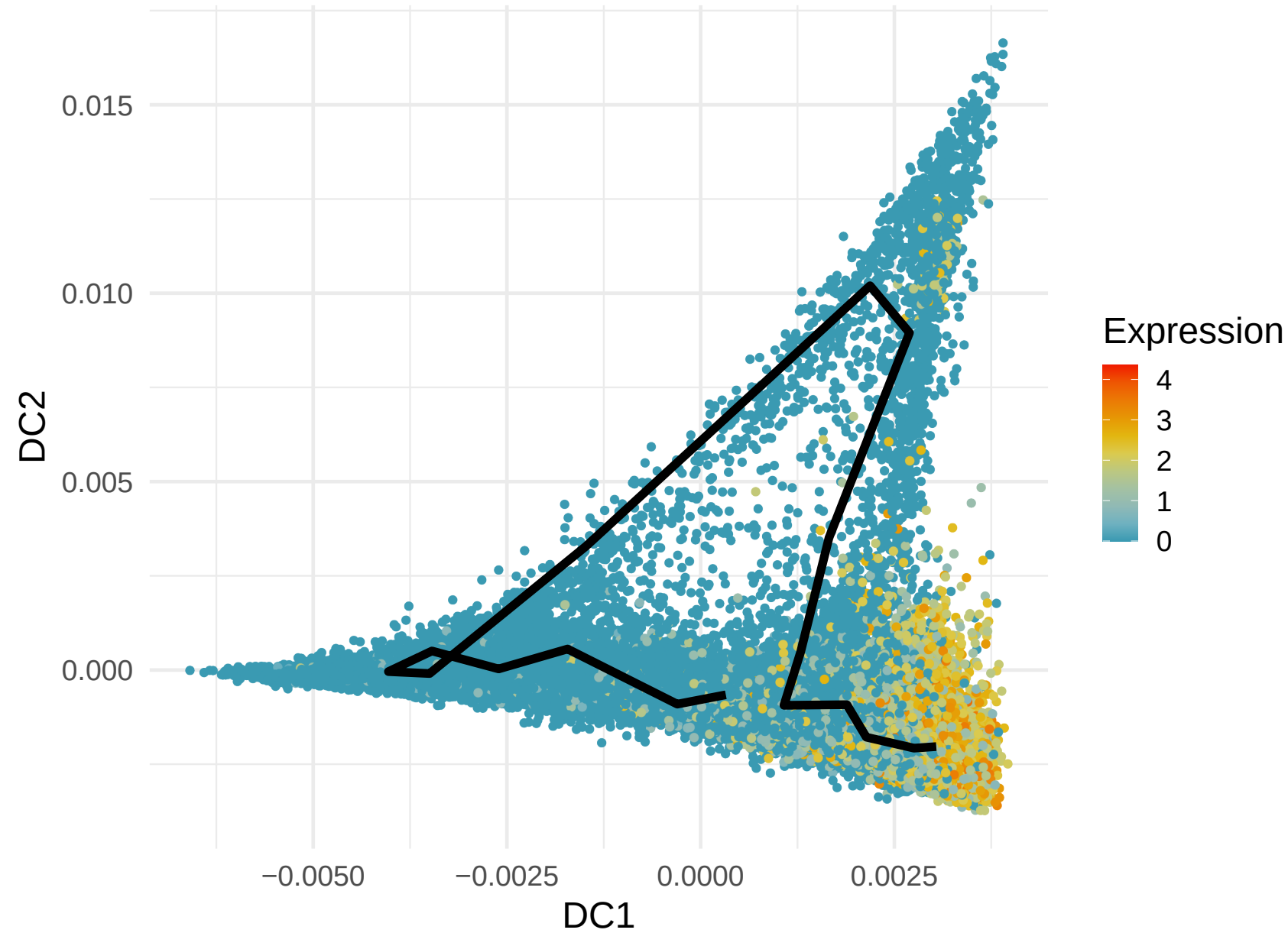
FGFBP2 Expression along Lineage 2 (R= 0.597)
