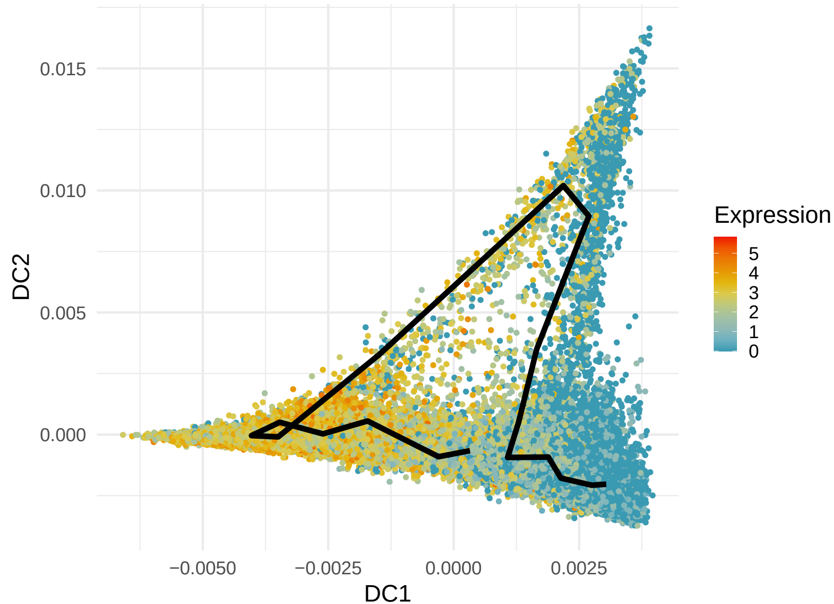
LTB Expression along Lineage 2 ( R = -0.506 )
