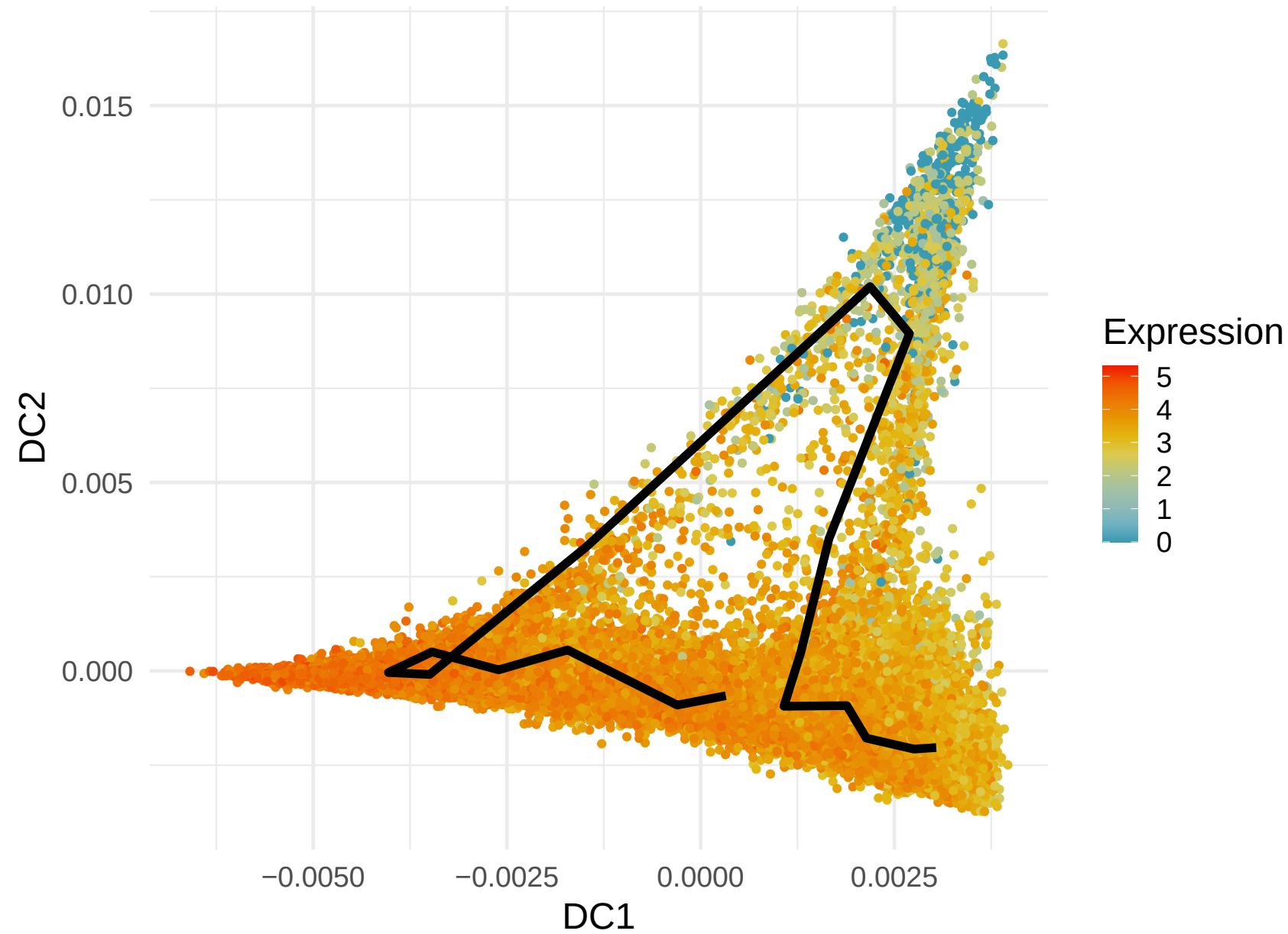
RPL34 Expression along Lineage 2 ( R = -0.318 )
