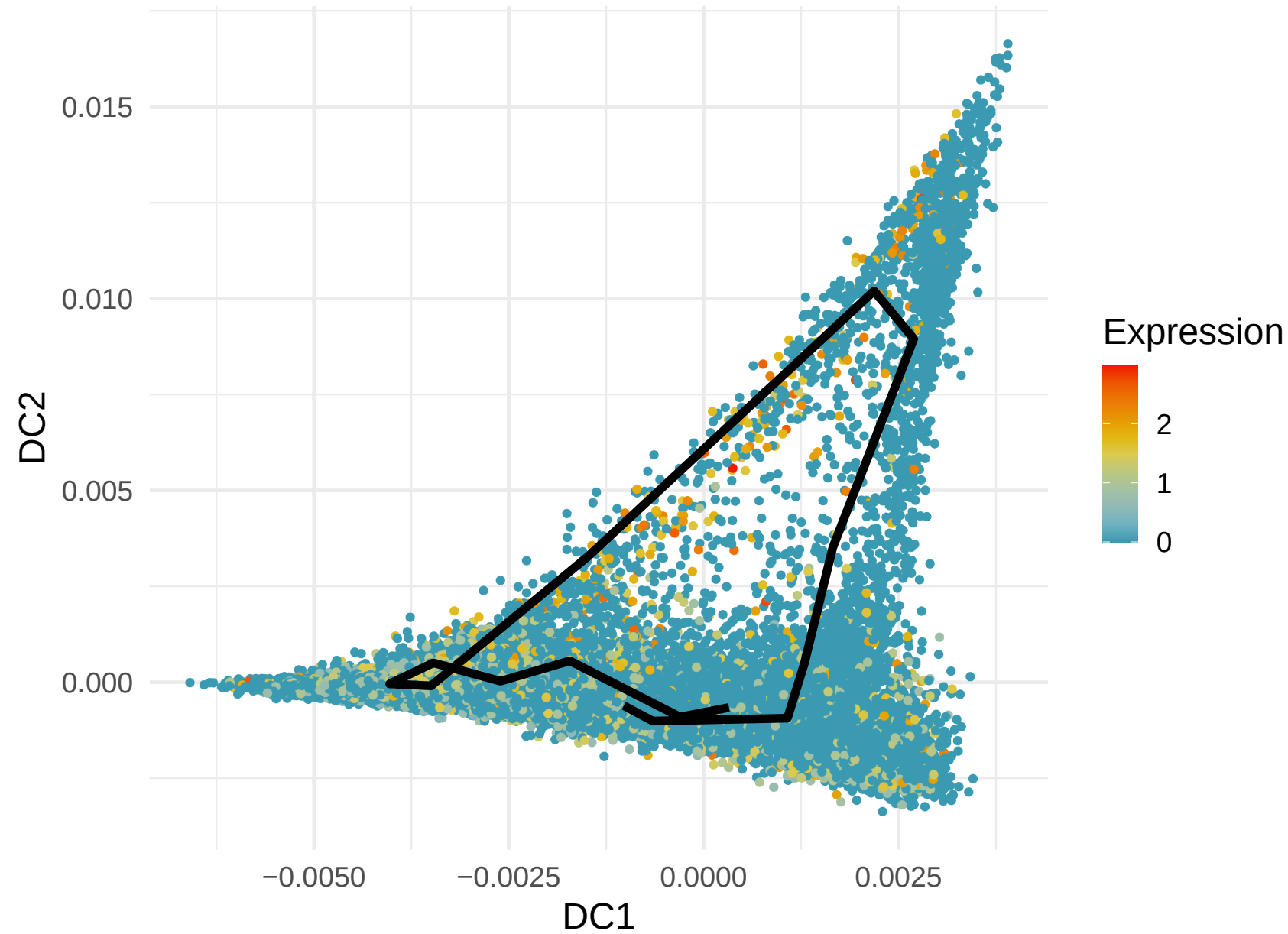
CD4 Expression along Lineage 3 ( R = -0.168 )
