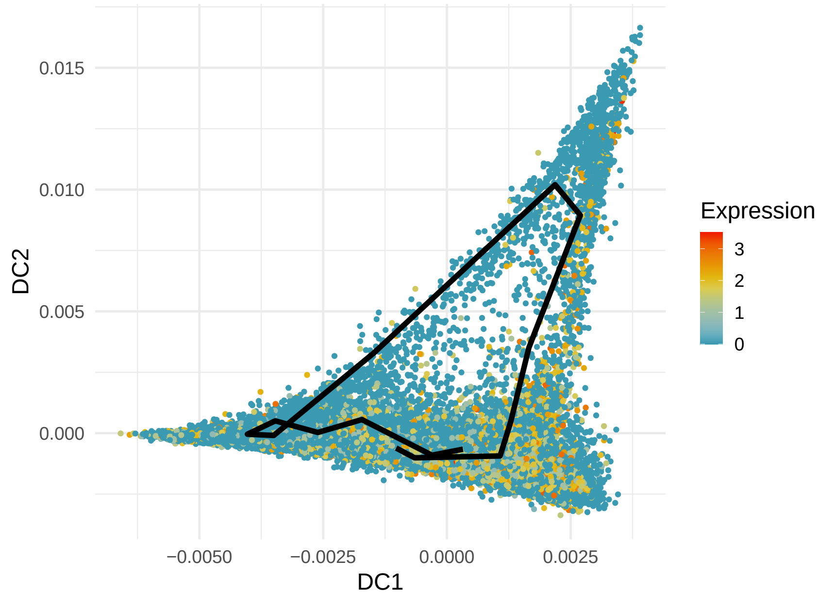
CD8B Expression along Lineage 3 ( R = 0.352 )
