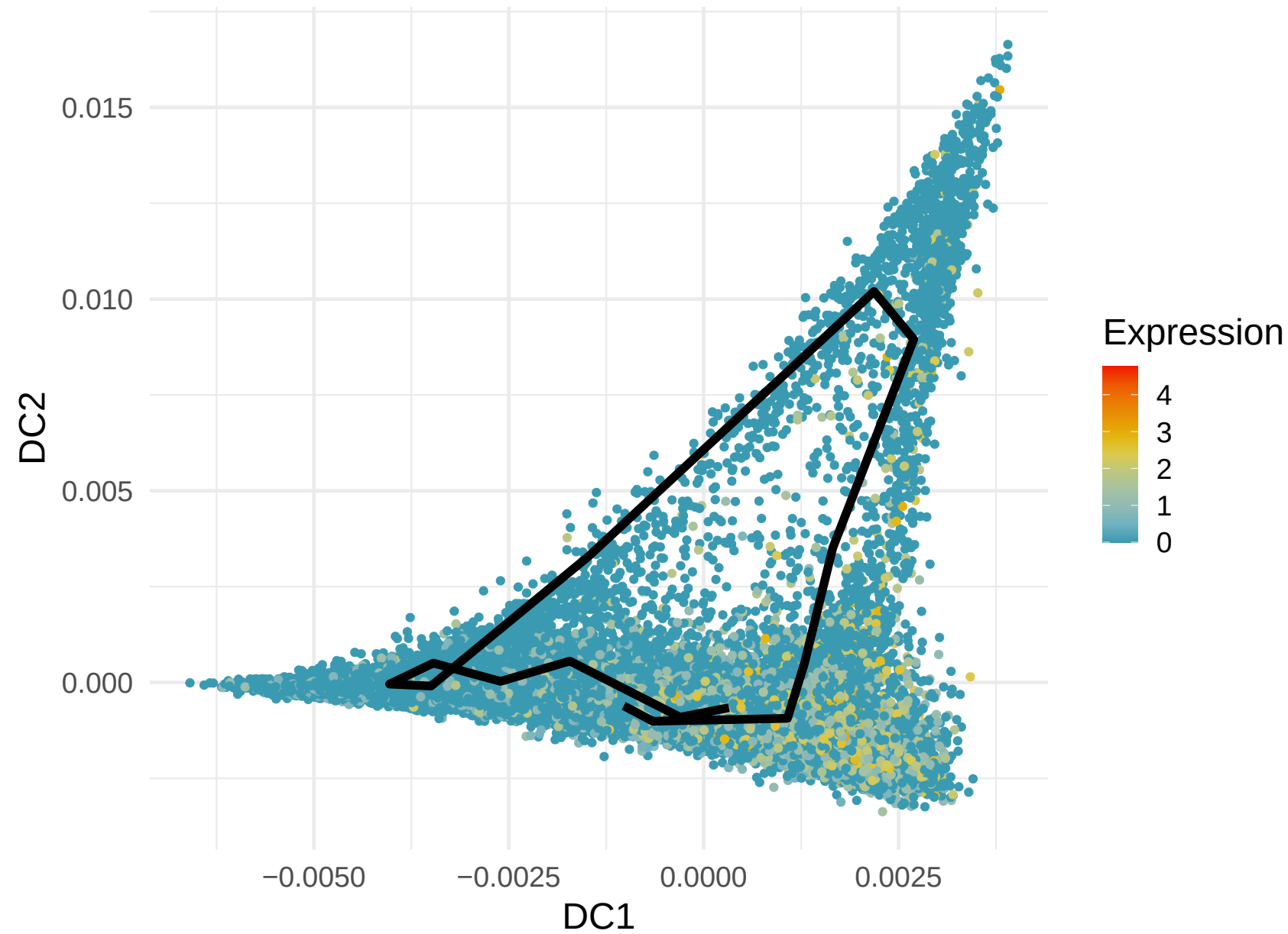
CMC1 Expression along Lineage 3 ( R = 0.211 )
